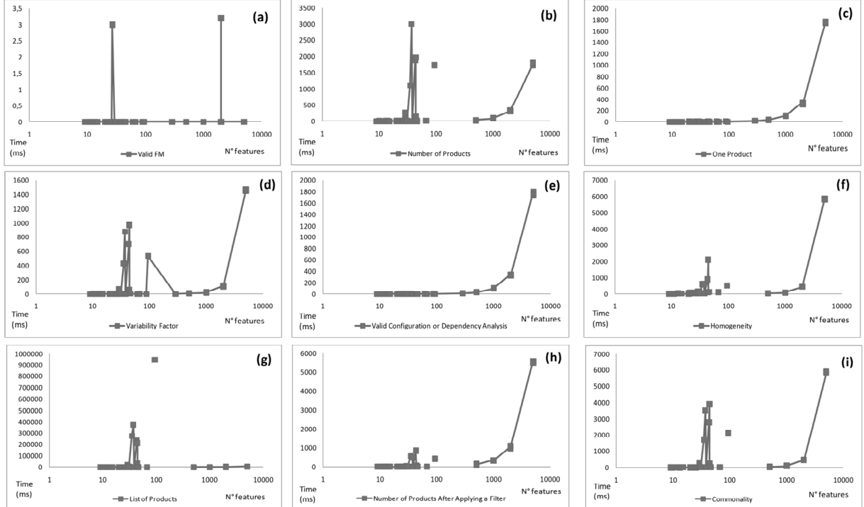
Figure 7. CPU time to execute our analysis operations over our 47 PLMs. Axe Y: time in milliseconds. Axe X Log 10 (Number of features)
