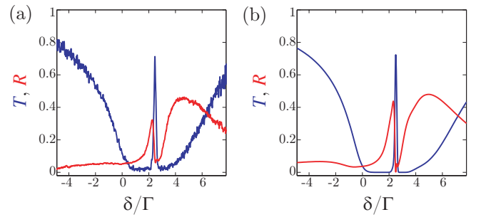
FIG. 5. (color online). Experimental (a) and simulated (b) transmission (blue) and reflection (red) spectra, with \Delta\lambda_{\text{lat}} = 0.13 nm, N = 1.5 \times 10^7 atoms, \eta = 3.5 and EIT parameters \Omega = 1.3\Gamma , \Delta = 2.5\Gamma , \gamma = 0.015\Gamma .
