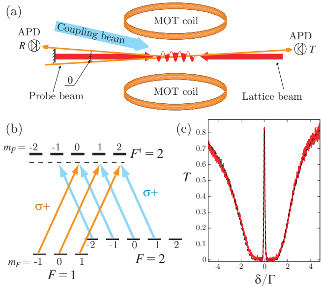
FIG. 4. (color online). (a) Scheme of the experimental setup. (b) Atomic levels and laser configuration. The probe (orange) and coupling field (blue) drive the transition F = 1 \rightarrow F' = 2 and F = 2 \rightarrow F' = 2 , respectively. (c) Transmission spectrum showing EIT with a disordered sample. The dashed black line is a fit to the data [Eqs. (1,11)], yielding the parameters \gamma = 7 \times 10^{-3}\Gamma , \Omega = 0.8\Gamma and optical thickness b_0 = 21 . The slight asymmetry is due to the cloud expansion during the sweep and is taken into account in the fit.
