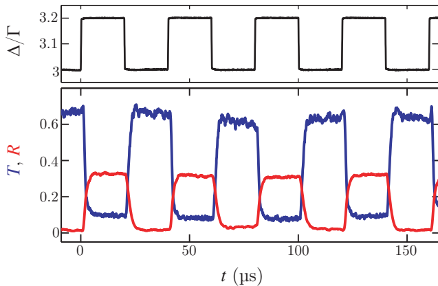
FIG. 8. (color online). Demonstration of a two-port all-optical switch. The detuning \Delta of the coupling field serves as the control parameter (top panel). The bottom panel shows the transmission (blue) and reflection (red) coefficients as a function of time. The control-field Rabi frequency is \Omega = 1.5\Gamma , the probe detuning is \delta = 3\Gamma and the lattice wavelength is such that \Delta\lambda_{\text{lat}} = 0.15 nm.
