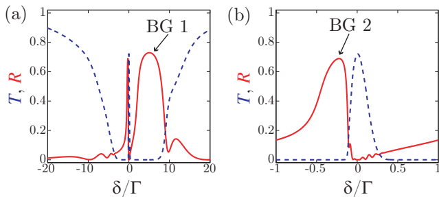
FIG. 3. (color online). (a) Computed transmission T (dashed blue line) and reflection R (red solid line) spectra with a lattice composed of N \sim 7700 periods. All other parameters are the same as for Fig. 2.
