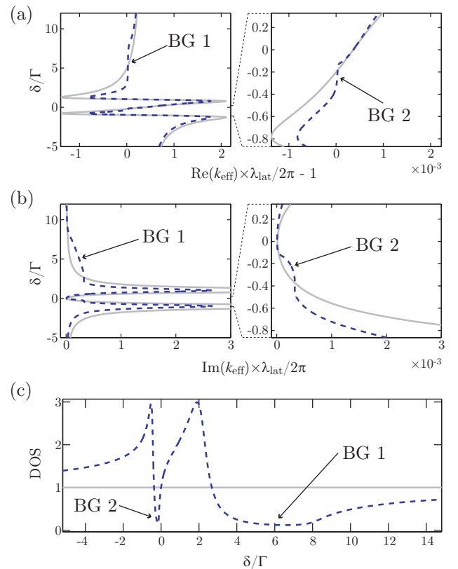
FIG. 2. (color online). Photonic properties of the medium, valid for an infinitely long lattice. (a) Dispersion relation: the frequency (detuning \delta ) is plotted as a function of the effective wavevector in the medium \text{Re}(k_{\text{eff}}) . Only the edge of the first Brillouin zone k_{\text{eff}}\lambda_{\text{lat}}/2 = \pi is shown. A first band gap (BG) is visible. Right panel: zoom in the transparency window, where a second BG appears. (b) Same as (a) with the imaginary part of k_{\text{eff}} . (c) Density of states (DOS) normalized to the one in a bulk medium of the same susceptibility [Eq. (10)]. In all plots, the grey solid lines correspond to a homogeneous atomic medium of the same average density \rho = 7 \times 10^{11} \text{ cm}^{-3} and the dashed blue lines correspond to atoms trapped in a lattice with \eta = 3.5 , \Delta\lambda_{\text{lat}} = 0.25 \text{ nm} and coupling-field parameters \Omega = 2\Gamma and \Delta = 0 .
