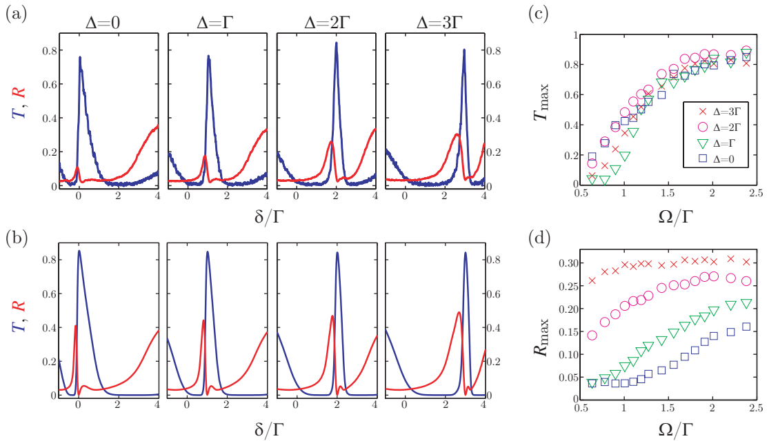
FIG. 6. (color online). Dependency on the EIT parameters, with a fixed lattice wavelength \Delta\lambda_{\text{lat}} = 0.11 nm. (a) Experimental transmission (blue) and reflection (red) spectra for several coupling-field detuning \Delta , with \Omega = 1.8\Gamma . (b) Corresponding simulations. (c) Maximum transmission in the transparency window as a function of the coupling-field Rabi frequency \Omega , for different detunings \Delta . (d) Same as (c) with the maximum reflection in the EIT reflection band.
