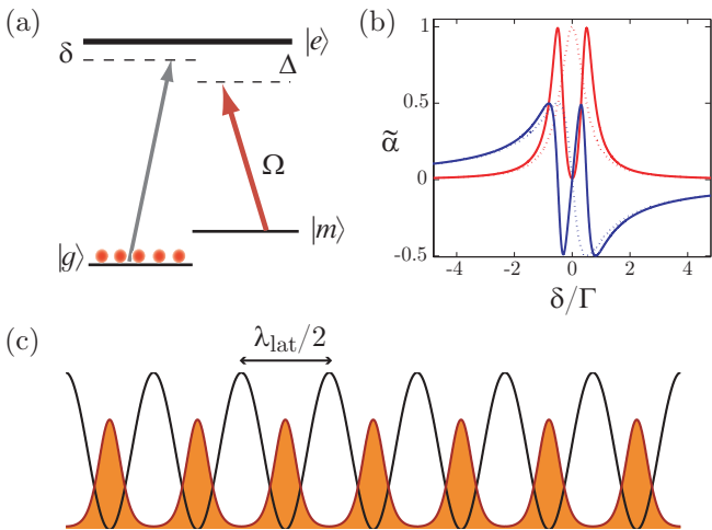
FIG. 1. (color online). (a) Atomic levels and laser configuration. (b) Real part (blue) and imaginary part (red) of the dimensionless atomic polarizability \tilde{\alpha} = \alpha \times \varepsilon_0 \hbar \Gamma / 2 |d_{ge}|^2 for a two-level atom (dotted lines) and with EIT (solid lines), with \Delta = 0 and \Omega = \Gamma [Eq. (1)]. (c) Scheme of the system under consideration: the atoms are trapped in a 1D optical lattice of periodicity \lambda_{\text{lat}}/2 .
