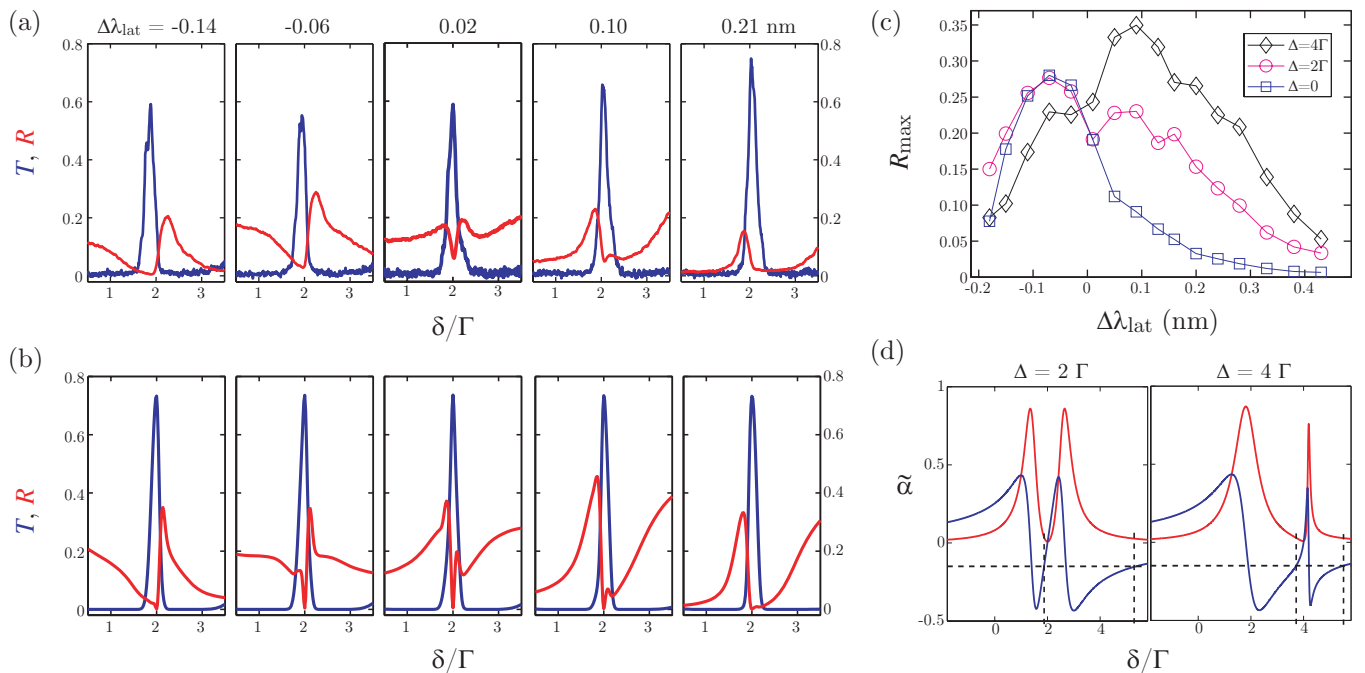
FIG. 7. (color online). Dependency on the lattice wavelength, with a fixed coupling-beam Rabi frequency \Omega = 1.3\Gamma . (a) Experimental transmission (blue) and reflection (red) spectra for several \Delta\lambda_{\text{lat}} and with a coupling-beam detuning \Delta = 2\Gamma . (b) Corresponding simulations. (c) Maximum reflection in the transparency window as a function of the lattice wavelength, for different detunings \Delta . (d) Illustration of the Bragg condition, which is fulfilled when the real part of the atomic polarizability (blue line) crosses the horizontal dashed black line representing -\Delta\lambda_{\text{lat}}/\lambda_{\text{lat}} [Eq. (2)]. The red line is the imaginary part of the atomic polarizability, proportional to scattering losses.
