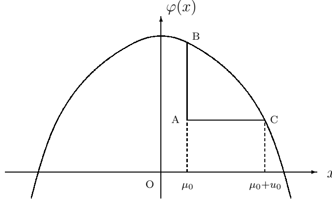
Figure 1. Graphical interpretation of Theorem 3.
