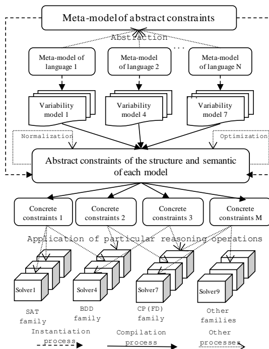
Figure 1: Constraint based configuration overview
