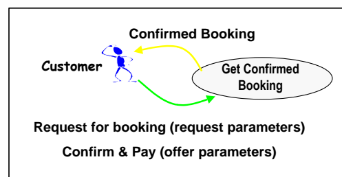
Figure 7: Booking interaction
