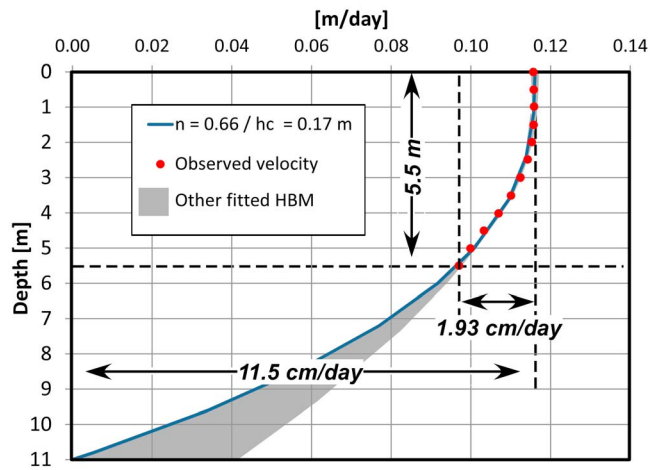
Figure 9. Red dots are observed displacement rates versus depth. Blue line represents velocity profile (corrected for the slope) computed from the Herschel-Bulkley model (HBM) with the fit parameters n = 0.66 , h_C = 0.17 m ( t_C = 1.4 kPa), and \mu_n = 1.7 \times 10^{9N} \text{ m}^{-2} \text{ s}^n . The shaded area shows all the HBMs fitting well the data (the coefficient of determination of the fitted law is r^2 = 0.98 ). The model giving the greatest velocity at the surface was chosen because it is closer to the observed surface velocities.
