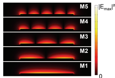
Fig. 5. Cross-section of the field-distribution (squared norm of the electric field) for 5 transverse modes sustained by the plasmonic waveguide.
