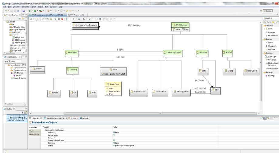
Fig. 10. BPMN metamodel in ecore using Obeco Designer
