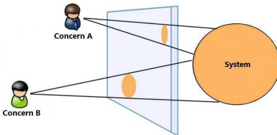
Fig. 11. Viewpoints notion
