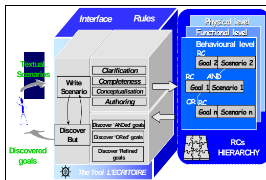
Figure 2: The L'Ecritoire architecture & functionality
