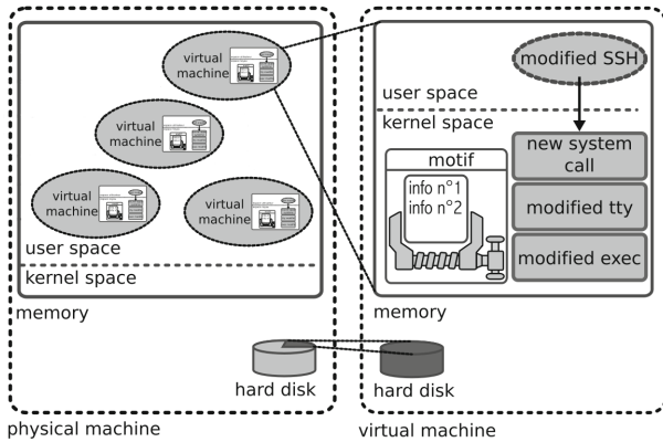
Fig. 1. Honeypot architecture
