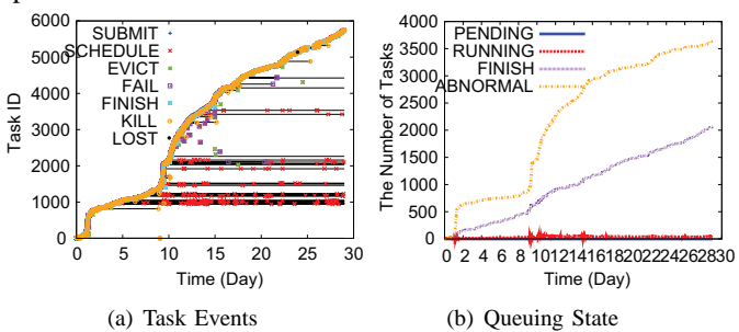
Figure 8. Task Events and Queuing State on a Particular Host
