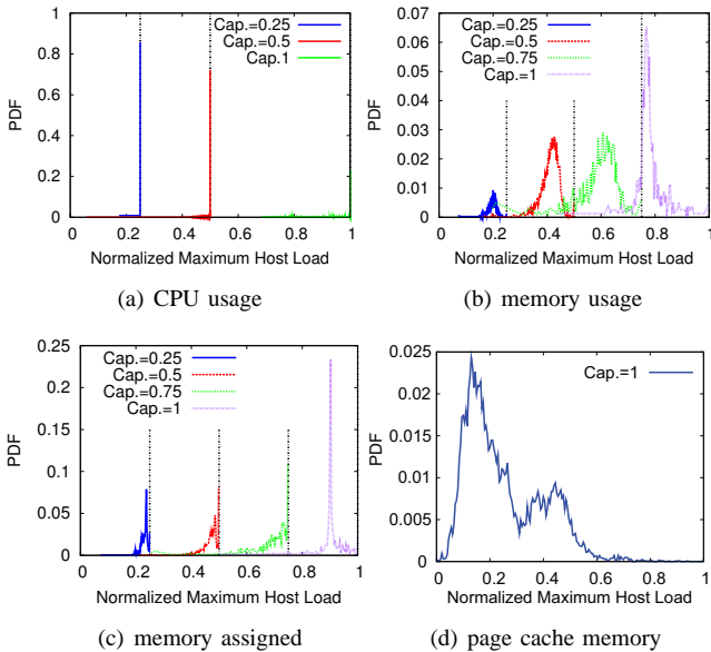
Figure 7. Distribution of Maximum Load
