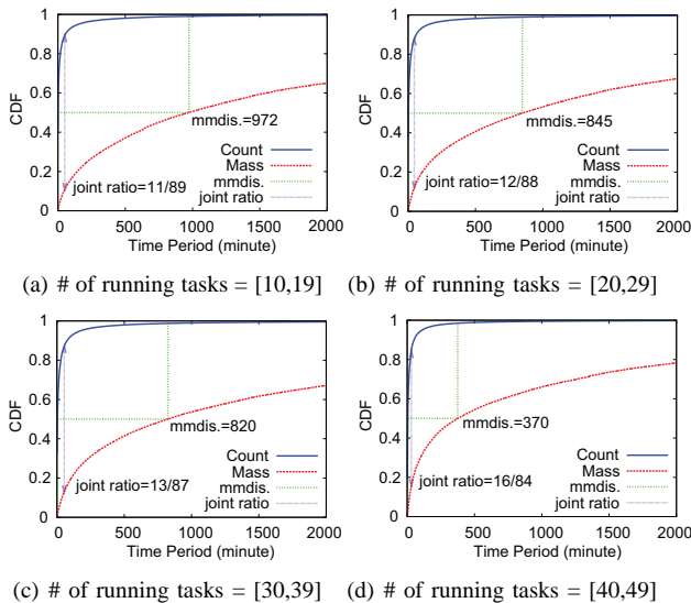
Figure 9. Mass-Count of Duration in Unchanged Queuing State
