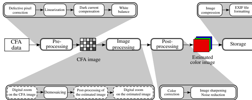
(b) Image acquisition in a single-CCD color camera (detailed diagram). Dotted steps are optional
