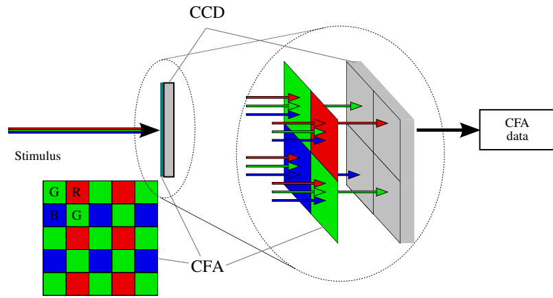
(a) Single-CCD technology (simplified), with filters arrangement according to the Bayer CFA
