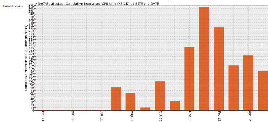
Figure 4.2: Site normalized CPU utilization per month
