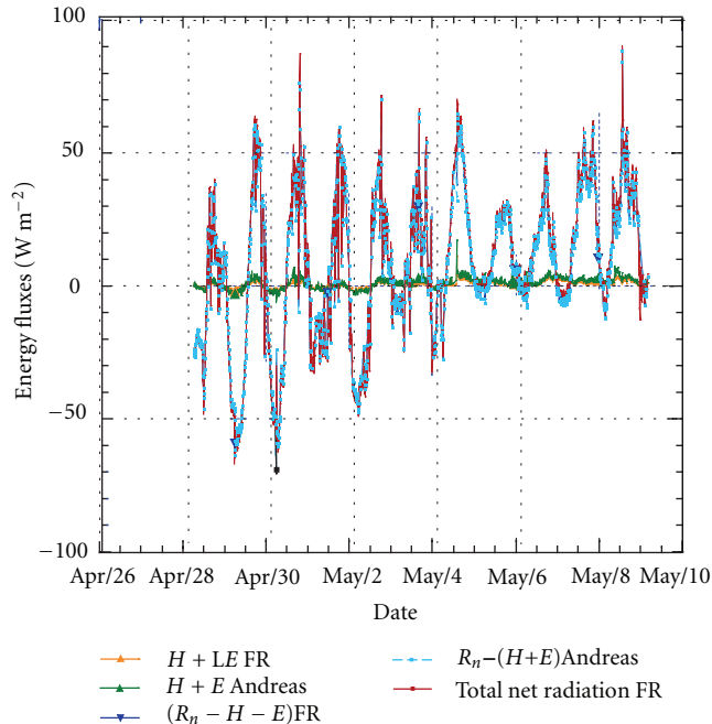
FIGURE 11: Temporal evolution of FR net radiation and turbulent bulk fluxes during the experiment. TR = R_n - (H + E) is also represented. The different bulk fluxes and TR using z_0 = z_{0t} = z_{0q} = 0.0001 m and [23] are also on the figure and quoted Andreas.
