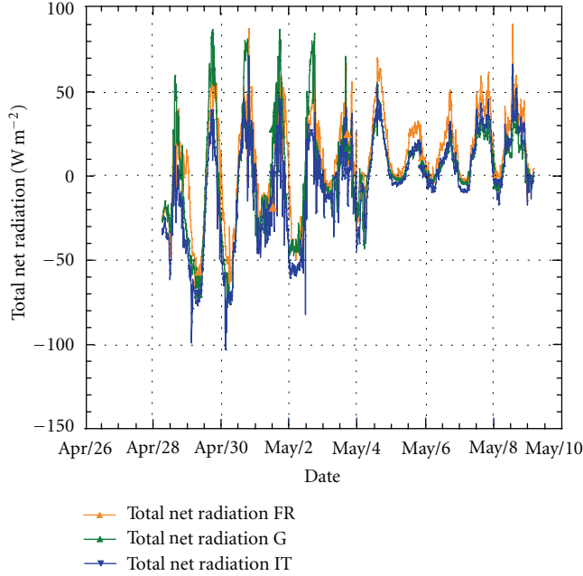
FIGURE 7: Evolution of net radiation during the experiment (FR, G and IT) from April 28 to May 9, 2010.
