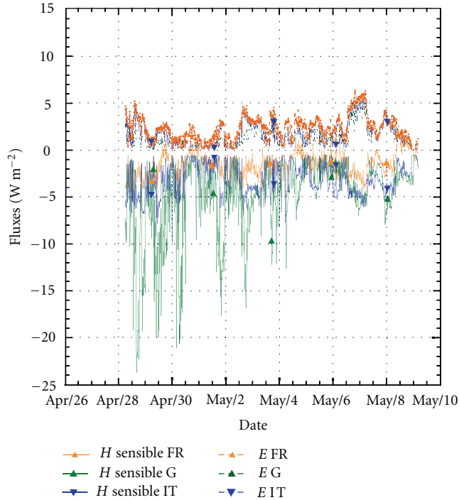
FIGURE 9: Estimates of the sensible heat flux H and latent heat flux E , obtained from the FR, IT, and G data for the period between April 28 and May 9, 2010.
