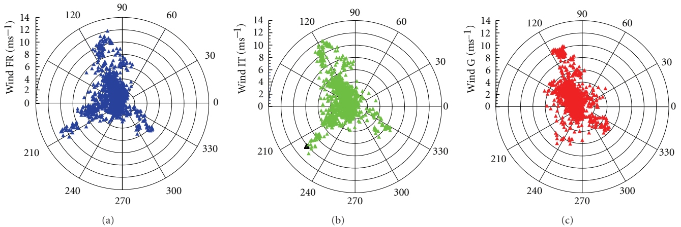
FIGURE 5: Windroses during the experiment from April 28 to May 8 (2010) for FR (in blue), IT (in green), and G (in red). We use conventional meteorological orientation (0 and 360 degrees for wind blowing from the north, 90 degrees for wind blowing from the east).
