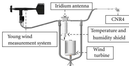
FIGURE 2: Conceptual scheme of the BEAR station.
