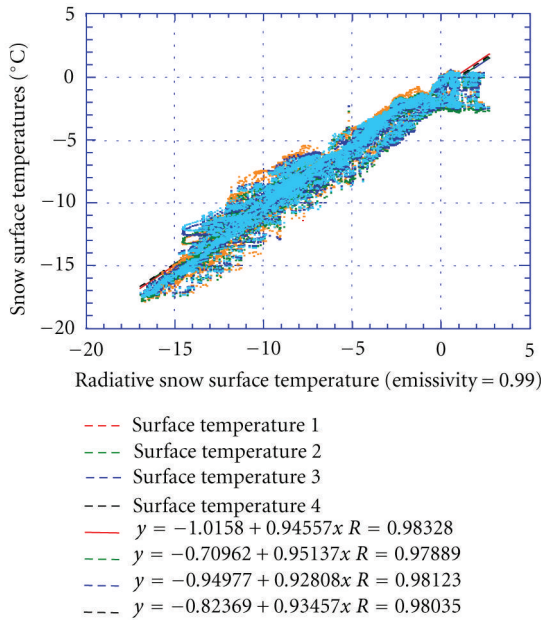
FIGURE 8: Scatter plot of surface temperature estimated from infrared radiation and the four temperature probes at 1.5 cm below the snow surface for a 0.99 surface emissivity.
