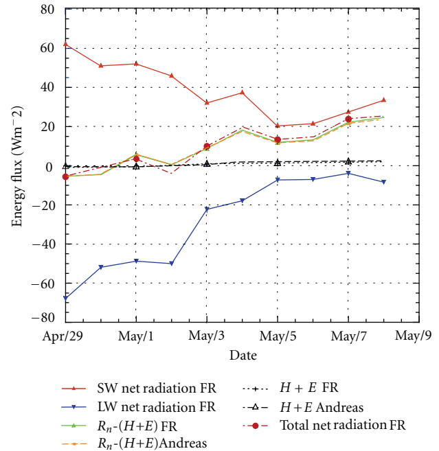
FIGURE 12: Daily averaged FR energy budget during the experiment, with each short-wave and long-wave net radiation components. TR is also drawn. The heat flux estimates are also plotted.
