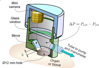
Figure 1 – LASTIC cross section: the upper part contains the camera while the lower part is the aspiration chamber with the mirror (left). Young moduli found by LASTIC and the tensile devices for each material (right).
