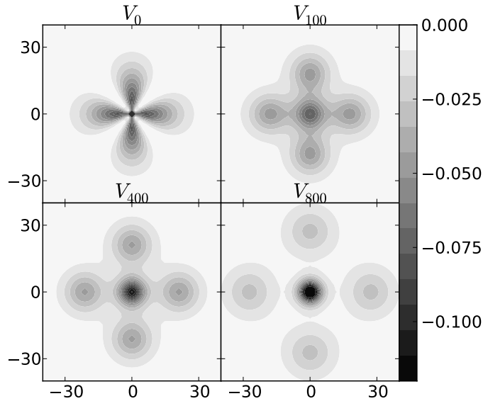
FIGURE 4. Separation in bumps of 2D non-radial initial data at \gamma = 1.2 , computed from Algorithm 1 with standard FEM. The initial data is taken to be a Gaussian in r multiplied by an angular factor (1 + \cos(4\theta)) .
