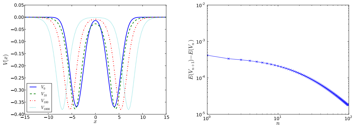
FIGURE 3. Divergence from a sum of Gaussian bumps at \gamma = 1.2 . Initializing to a single Gaussian of large width yields similar results. The two bumps separate slowly, until the finiteness of L forces convergence. Although not displayed here, the asymptotic logarithmic divergence (11) can be checked graphically, e.g. the spacing between V_{100} and V_{1000} is the same than between V_{1000} and V_{10000} . The asymptotic slope of the log-log convergence plot is -1 , which fits with the heuristic arguments given.
