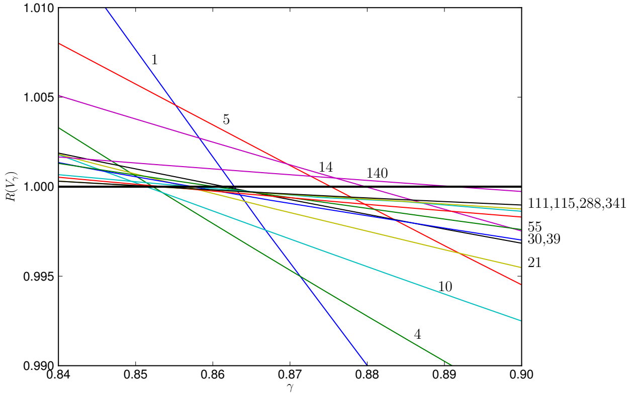
FIGURE 7. R(V) as a function of \gamma for d = 3 , with the same methodology as in Figure 5. As \gamma increases, different branches become maximizers, until \gamma = 1 . The fact that only some branches are above the threshold R = 1 when the number of bound states increases results from the highly oscillatory behavior near \gamma = 1 , as predicted in [8].
