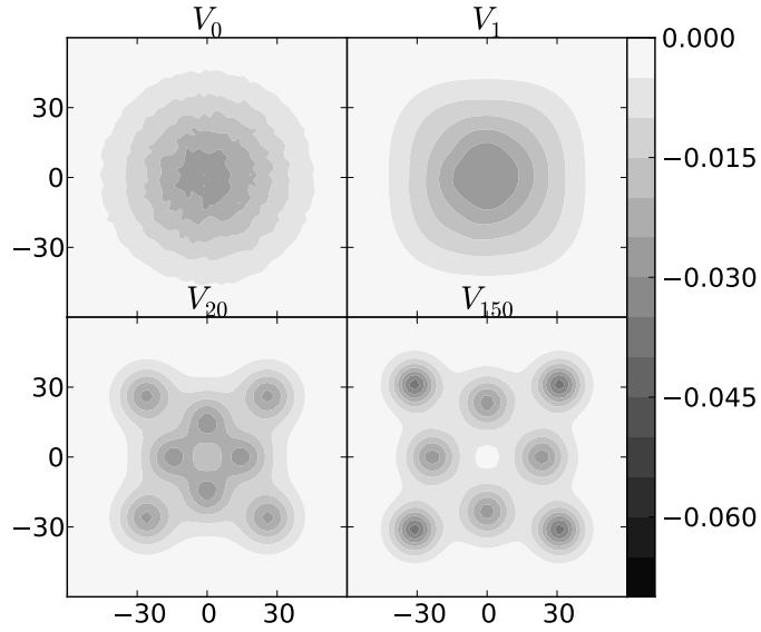
FIGURE 6. Separation in bumps of the randomly perturbed radial potential with eight bound states, \gamma = 1.1 .
