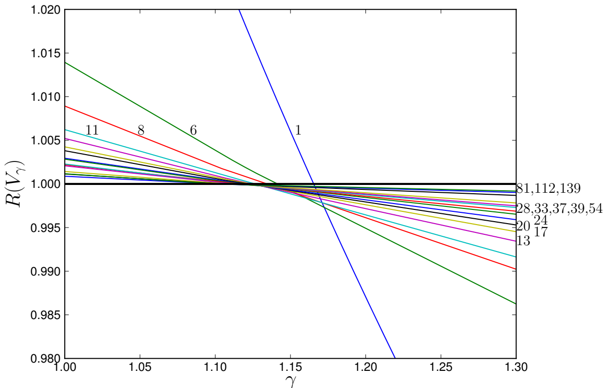
FIGURE 5. R(V) as a function of \gamma for d = 2 using the branch continuation procedure in the radial setting (Algorithm 2). The branches are labeled by the number of bound states they have. Based on these results, the maximizer seems to be V_{\gamma,d,1} , up to \gamma \approx 1.16 . Above this, no branches were above the semiclassical regime R = 1 .
