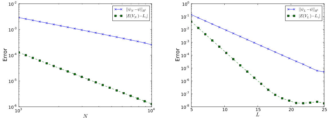
FIGURE 1. Convergence analysis with respect to N and L . The figure on the left illustrates the convergence of the eigenfunctions and eigenvalues with respect to the number of grid points N , with a fixed L = 40 , large enough to cause a negligible error. The slopes, found by linear regression, are -1.043 for the eigenvectors and -1.999 for the eigenvalues, close to their theoretical values of -1 and -2 . The figure on the right illustrates the convergence of the eigenfunctions and eigenvalues with respect to the domain size, with constant stepsize h = 5 \times 10^{-4} . The slope for the eigenvectors is -0.5285 \approx \sqrt{-\lambda} = -0.5283 . When the domain size gets large enough, the error due to h dominates, and causes a plateau.
