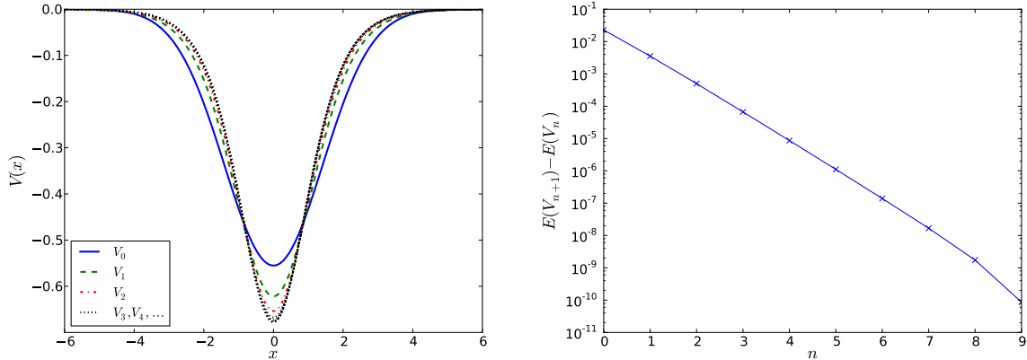
FIGURE 2. Linear convergence from a Gaussian initial data towards V_{\gamma,d,1} . This plot is for \gamma = 1.2 .
