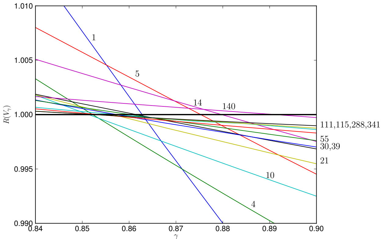
FIGURE 7. R(V) as a function of \gamma for d = 3 , with the same methodology as in Figure 5. As \gamma increases, different branches become maximizers, until \gamma = 1 . The fact that only some branches are above the threshold R = 1 when the number of bound states increases results from the highly oscillatory behavior near \gamma = 1 , as predicted in [8].
