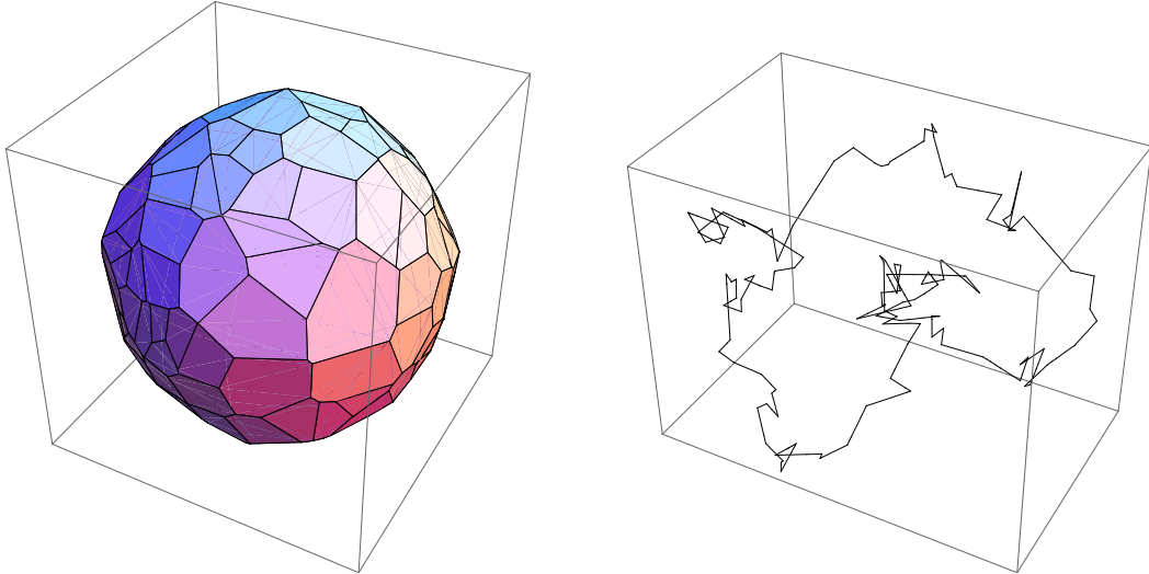
Figure 1: On the left: tessellated surface determined by the areas and normals of its facets; typical configuration belonging to the ensemble with fixed total area discussed in the text ( A_H \approx 100 L_P^2 ). On the right: closed polymer chain corresponding to the tessellated surface.
