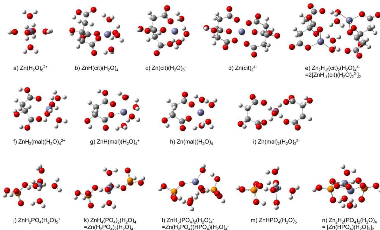
Figure 1. Molecular structures of hydrated Zn^{2+} and aqueous Zn citrates, malates, and phosphates. Structures are drawn by using GaussView5 (Gaussian Inc.) [14]. Symbols are: Zn (iris), P (orange), O (red), C (gray), and H (white). doi:10.1371/journal.pone.0030726.g001
