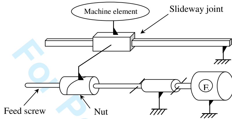
Fig. Axis guiding system of the machine
