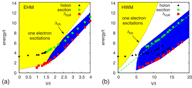
FIG. 3. (Color online) Excitation spectra for the models with (a) nearest-neighbor (EHM) and (b) long-range interactions (HWM) on L=16 sites. The symbols represent respectively the holon (triangles) and exciton (dots) peaks in the optical conductivity, and the lowest excitation of finite energy as given by the ED (squares). The light shaded (yellow) region is delimited by the single-particle charge gap \Delta_{ch} , while the dark (blue) region corresponds of the collective excitations of the Wigner lattice, bounded from below by \Delta_{coll} . The dashed line is predicted exciton energy in the thermodynamic limit, 0.62V (see Appendix A).
