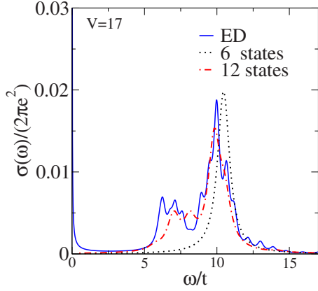
FIG. 8. (Color online) Comparison of the optical conductivity calculated at V=17t from ED of a L=16 cluster to the one obtained from the defect model, including respectively the 6 and 12 lowest-lying states.
