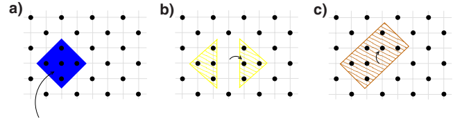
FIG. 9. (Color online) The lowest-lying states with one electron added to the perfect checkerboard pattern. From left to right the corresponding Madelung energies in an infinite system are (a) E_I = 0.8078V , (b) E_D = 0.9233 and (c) E_D = 1.1304
