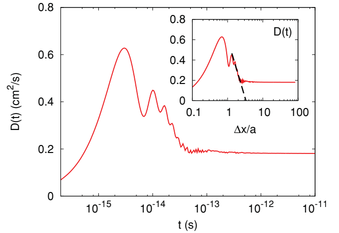
FIG. 2. (Color online) Time-dependent electron diffusivity D(t) extracted via Eq. (4) from the experimental optical conductivity of Ref. 16 in the direction of highest conduction. The absolute value is fixed by the measured mobility \mu \simeq 7 \text{ cm}^2/\text{Vs} . The inset shows the same quantity as a function of the instantaneous electron spread. The dashed line is the weak localization extrapolation.
