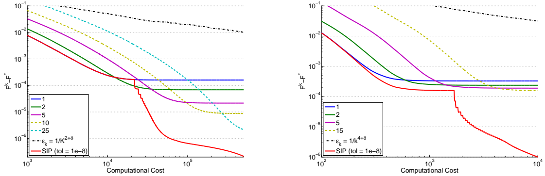
Figure 2: Deblurring with Total Variation - Basic method (left) and Accelerated method (right)
