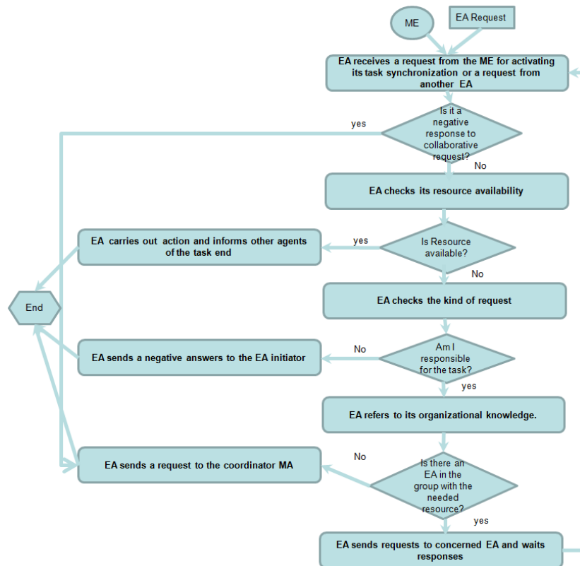
Fig. 10 EA synchronization behaviour (Tounsi et al. 2009a)
