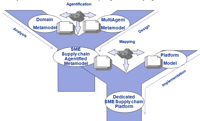
Fig. 1 ArchMDE development process (Tounsi et al. , 2009c)
