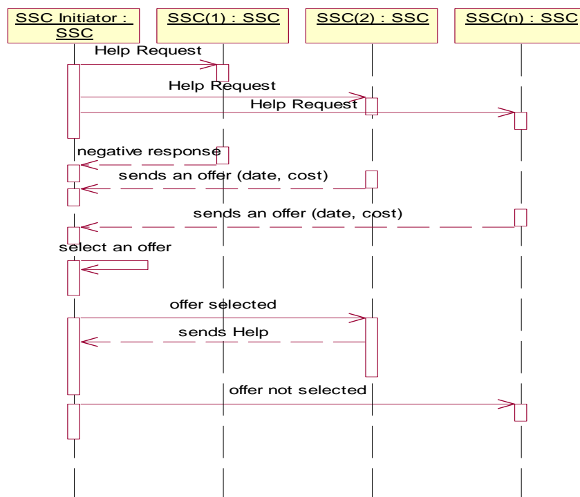
Fig. 11 SSC coordination process (Tounsi et al. , 2009b)
