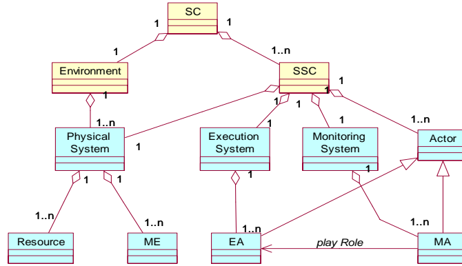
Fig. 6 Intermediary domain metamodel (Tounsi et al., 2009c)
