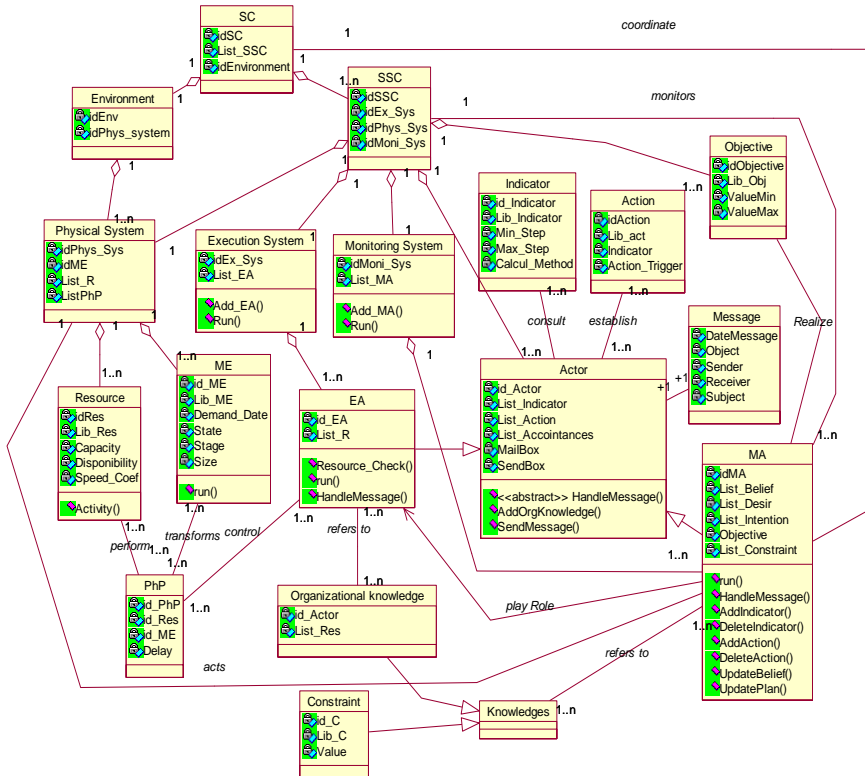
Fig. 13 The Implementation Metamodel (Tounsi et al. , 2011)
