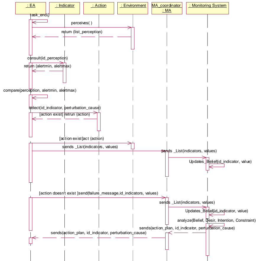
Fig. 12 Sequence diagram of the monitoring and control protocol ( Tounsi et al., 2011 )
