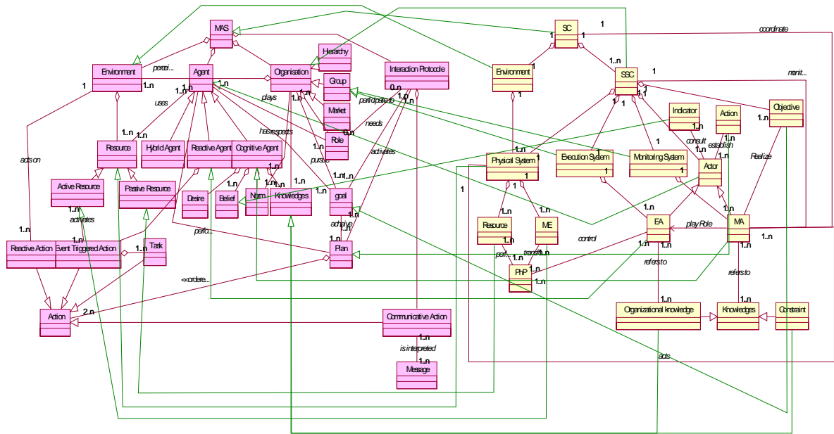
Fig. 9 The agentified SME supply chain metamodel (Tounsi et al. , 2009c)
