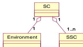
Fig. 4 Abstract domain metamodel (Tounsi et al. , 2009c)
