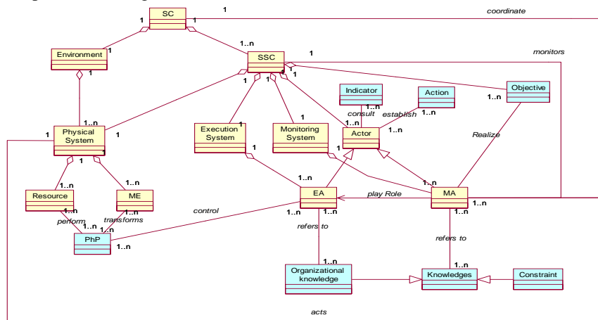
Fig 7. Final domain metamodel (Tounsi et al., 2009c)
