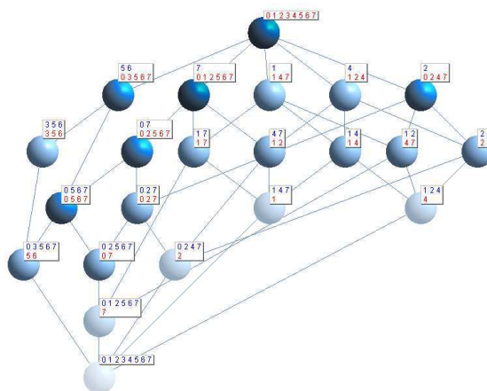
Fig. 7. The Galois Lattice of Social Network shown in the figure 6.
