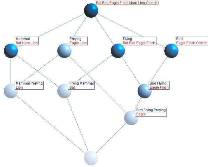
Fig. 5. Species Galois Lattice.
