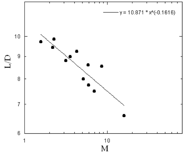
Figure 6: Logarithmic plot of the ratio L/D as a function of M . The equation of the power law fit shows a much slower decrease than the M^{-1/2} scaling predicted by Raynal (1997).
