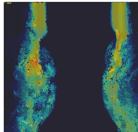
Figure 12: PIV visualization of the gas velocity field around the liquid jet: the flow is non axisymmetric. U_g = 10 m/s and U_L = 0.4 m/s.
