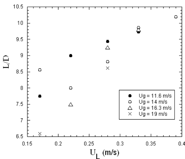
Figure 5: Liquid intact length L of the jet nondimensionalized by the liquid injector diameter D , as a function of liquid and gas velocity.
