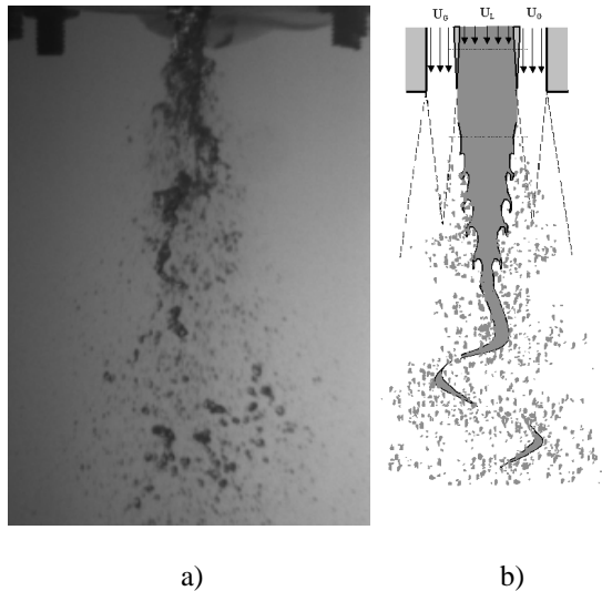
Figure 4 : a) Airblast atomization for U_G = 40 m/s and U_L = 0.3 m/s ; b) sketch emphasizing how the flapping instability creates large liquid fragments.
