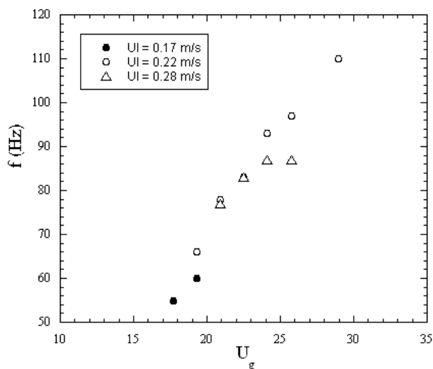
Figure 9: Frequency of the flapping instability as a function of gas velocity, for different liquid velocities.
