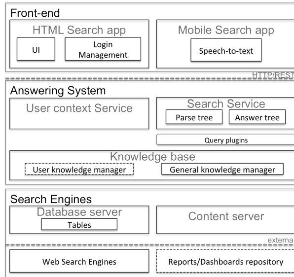
FIG. 1 – Architecture of the answering system
