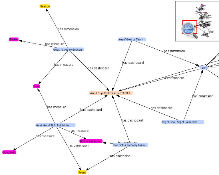
Fig. 2. Graph describing a dashboard (orange) and associated charts (blue), with referenced measures (purple) and dimensions (yellow).
