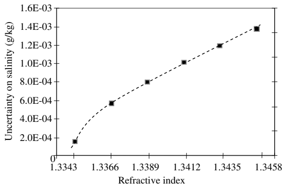
Figure 4. Assessment from a theoretical functioning model of the uncertainty linked to the variation of the refractive angle on salinity measurements as a function of the medium refractive index. The refractive angle decreases when salinity increases.
