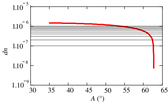
Figure 2. Sensitivity of seawater refractive index to incident angle A .
