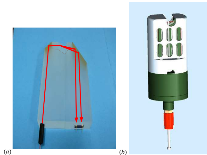
Figure 5. (a) Optical part with the laser on the left and the PSD on the right. The two beam paths correspond to the refractions obtained with seawater on the left and with distilled water on the right. (b) NOSS sensor containerization. At the top part of the instrument, the measurement area is visible with the external temperature sensor contained in a long stainless steel rod. At the bottom part, there are the electronic container and the connector.
