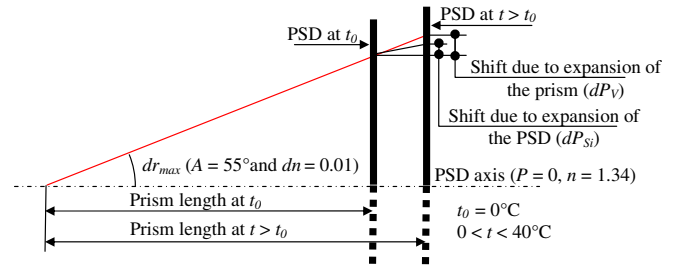
Figure 3. Positioning error due to prism and PSD expansion.
