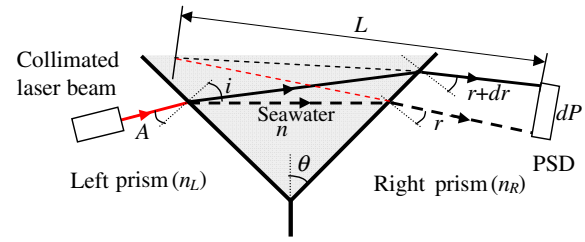
Figure 1. Schematic diagram of TPR.
