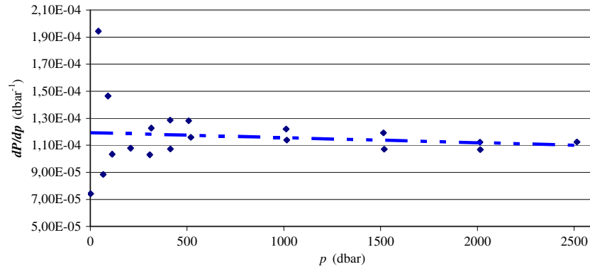
Figure 6. Dots represent the sensitivity of the PSD position ( P ) as a function of pressure ( p ) applied during the experiment in the pressure tank. The straight line is the average correction applied to the data. Under 500 dbar, the position data show an increasing discrepancy due to the inaccuracy of the corrections applied to the measured P . These corrections are necessary because the salinity decreased by 0.059 and the temperature by 1.508 °C during the measurements. But, by applying an average sensitivity dP/dn = 81.431 on the residual position errors, these discrepancies correspond only to maximal residual errors of 9 \times 10^{-7} for increasing pressures and -5 \times 10^{-7} for decreasing pressures, on the index.
