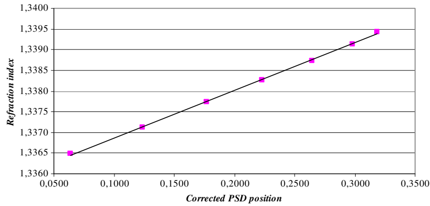
Figure 7. Result of the calibration of the corrected PSD positions as a function of the refractive index. The relation is found to be very linear (Pearson correlation sampling coefficient r^2 = 0.9992 ).
