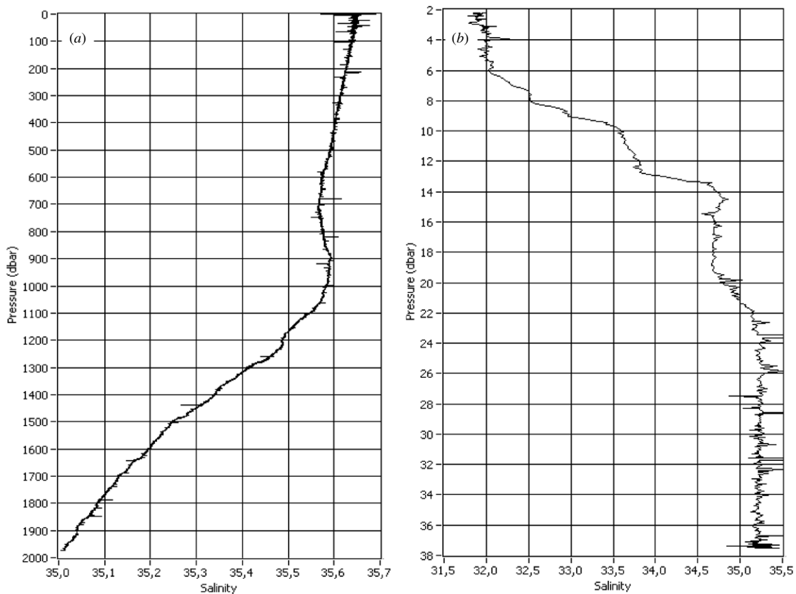
Figure 8. Examples of index profiles obtained during an oceanographic campaign in the Bay of Biscay. (a) A 2000 m depth profile that has been realized in an area where density variations are mostly due to temperature variations. Acquired at the frequency of five samples per second, it has been expressed in salinity by inverting the Millard and Seaver algorithm. (b) A profile obtained in a coastal area where density variations are mostly due to salinity variations. The two profiles are unfiltered and the response times of the index, temperature and pressure sensors have not been aligned, which can explain the visible spikes.
