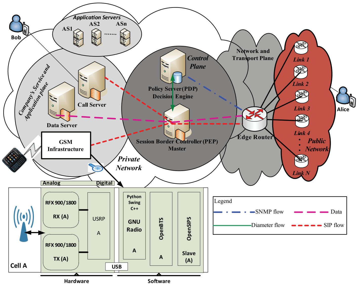
Fig. 1. Proposed Architecture.
