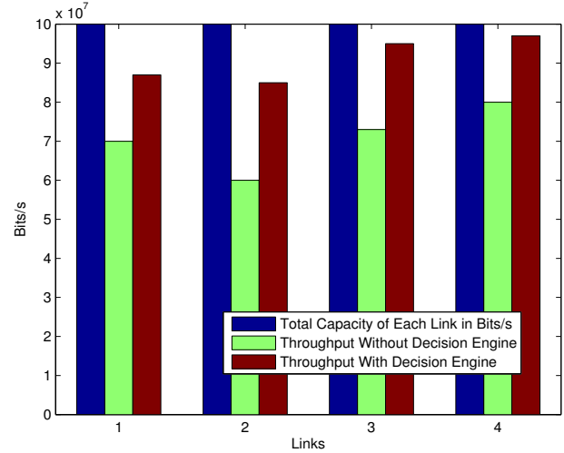
Fig. 6. Throughput of Each Link With and Without Decision Engine.
