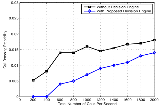
Fig. 7. Call Dropping Probability With and Without Decision Engine.
