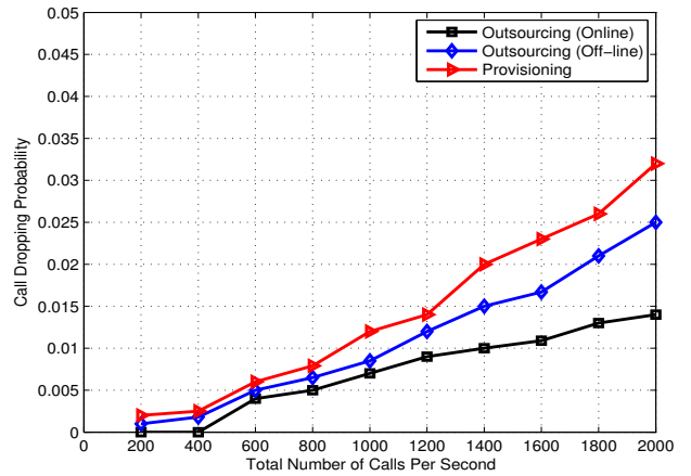
Fig. 10. Call Dropping Probability Introduced by the System in Outsourcing (Online and Off-line) and Provisioning Mode Respectively.
