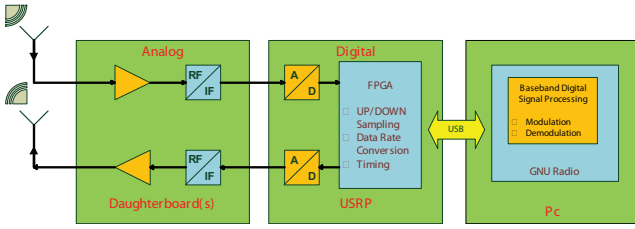
Fig. 2. Software Defined Radio Block Diagram.
