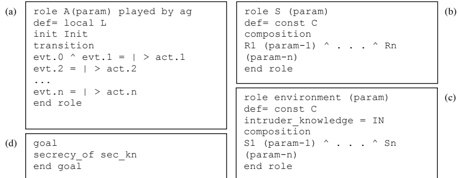
Fig. 1. HLPSL main elements. (a) Basic role structure. (b) Session role structure. (c) Environment role structure. (d) Secrecy in the goal section.
