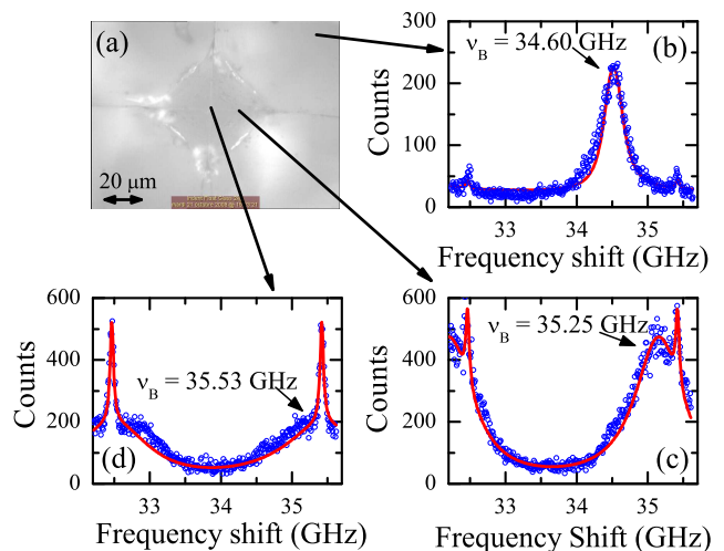
FIG. 2. (Color online) a) Top-view photograph of a 2-kg Vickers indent on a soda-lime silicate glass surface. b-d) Brillouin spectra taken at 5 \mu\text{m} beneath the surface, for a pristine sample volume far from the indented area, along the edge of the Vickers indenter at 12 \mu\text{m} from the center and at the center, respectively.
