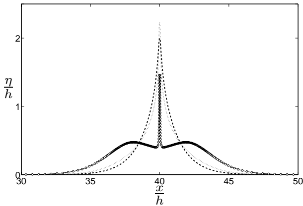
Fig. 8. Rundown for initial amplitude a/h=0.70 : Residual jet formation; \cdots t/\tau=16 ; --- t/\tau=17 ; - - - t/\tau=18 ; \circ t/\tau=18 .
