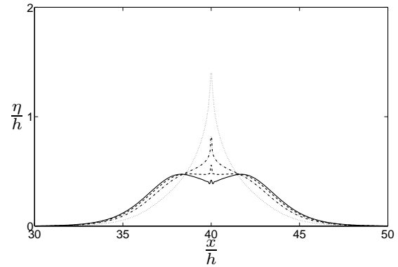
Fig. 10. Rundown for initial amplitude a/h=0.60 : Residual jet ; \cdots t/\tau=17.5 ; --- t/\tau=18.1 ; - - - t/\tau=18.3 ; - t/\tau=18.4 .
