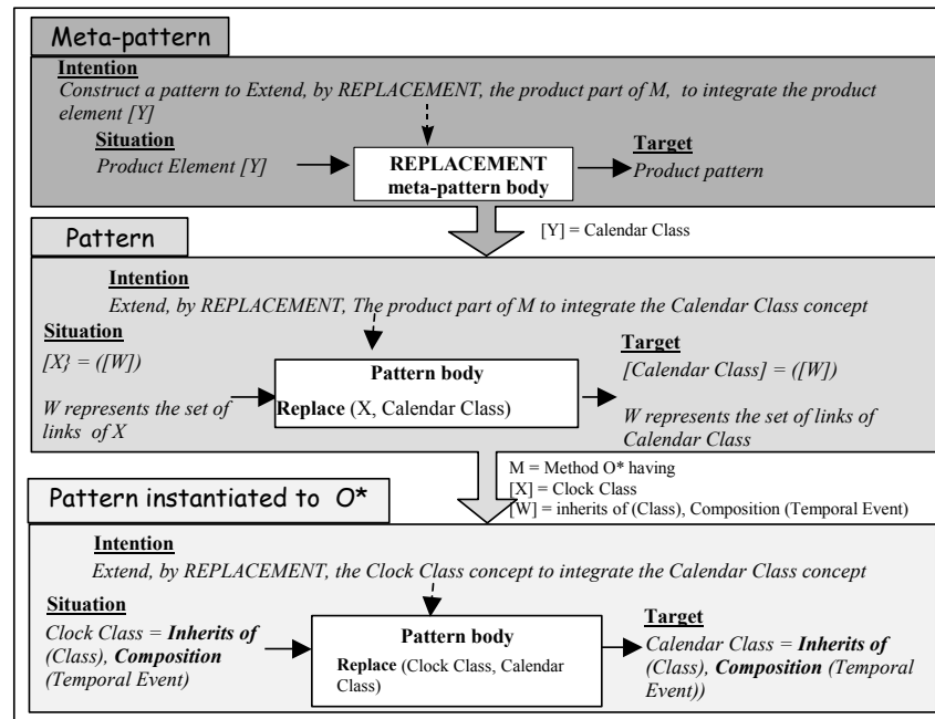
Figure 4: Example of pattern construction with meta-patterns
