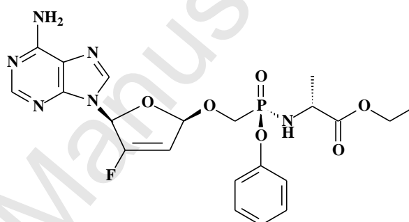
GS-9131 (Fd4A phosphonoamidate)
