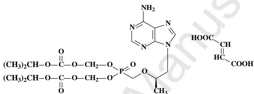
31 32 33 34 35 Tenofovir disoproxil fumarate (TDF)
