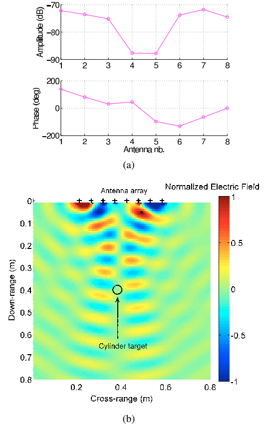
Fig. 5. UWB D.O.R.T. experiment. Anti-symmetric singular vector (associated to \lambda_2 in Fig. 4) (a) complex law and (b) real part of the corresponding monochromatic field chart at 3 GHz.
