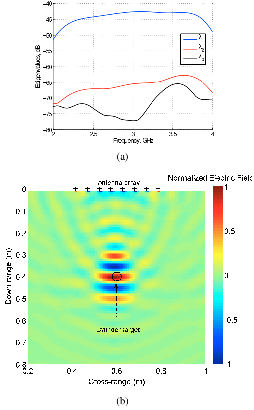
Fig. 4. UWB D.O.R.T. experiment. (a) Array inter-element matrix eigenvalues distribution versus frequency and (b) one frame of the synthetic time-domain field chart movie associated to the largest eigenvalue.
