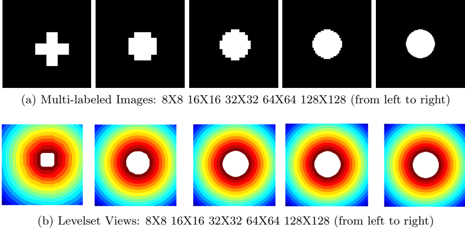
Figure 7: Voxel-based geometry and X-FEM geometry
