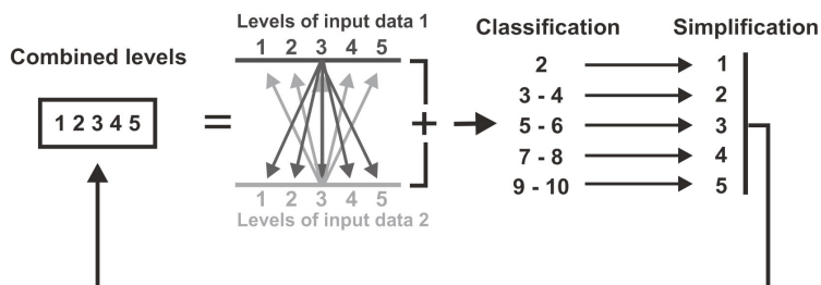
Fig. 3. Levels of erosive pressure and combination procedure in the SCALES model
