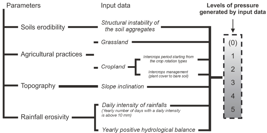
Fig. 2. Types of parameters and input data and levels of pressure concerning soil erosion
