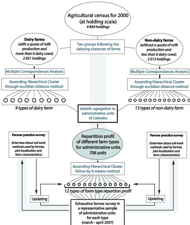
Fig. 5. Procedure for characterizing the agricultural practices in Calvados
