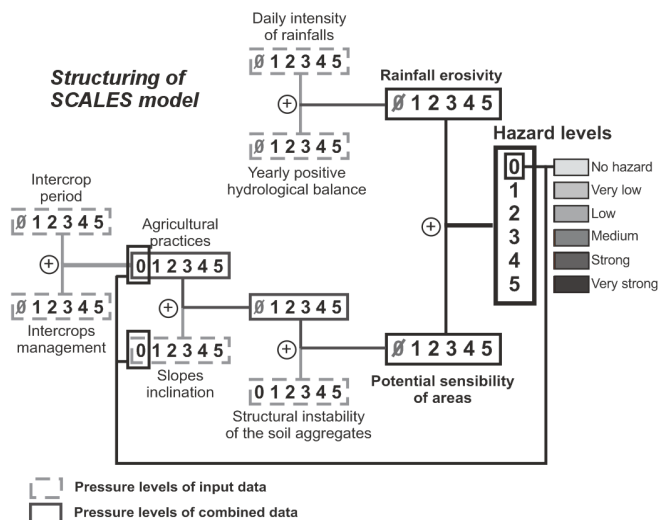
Fig. 4. Defining hazard levels using SCALES model
