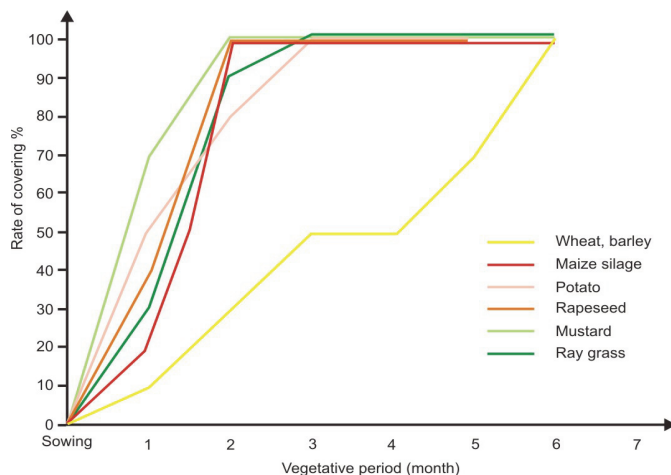
Fig. 8. rate of covering according to the vegetative period of various cultures (Arvalis)
