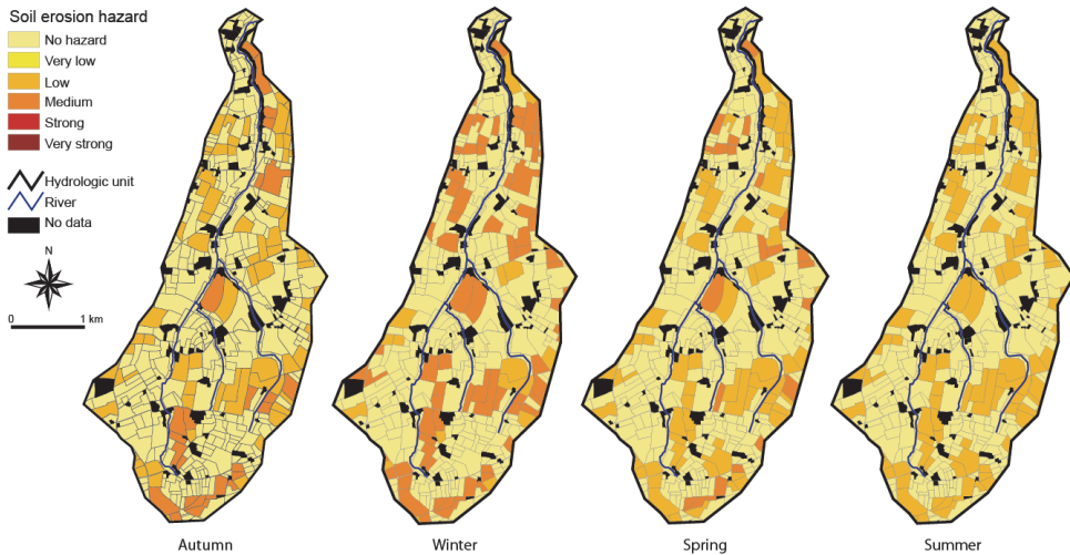
Fig. 10. Maps of soil erosion hazard at seasonal scale.
