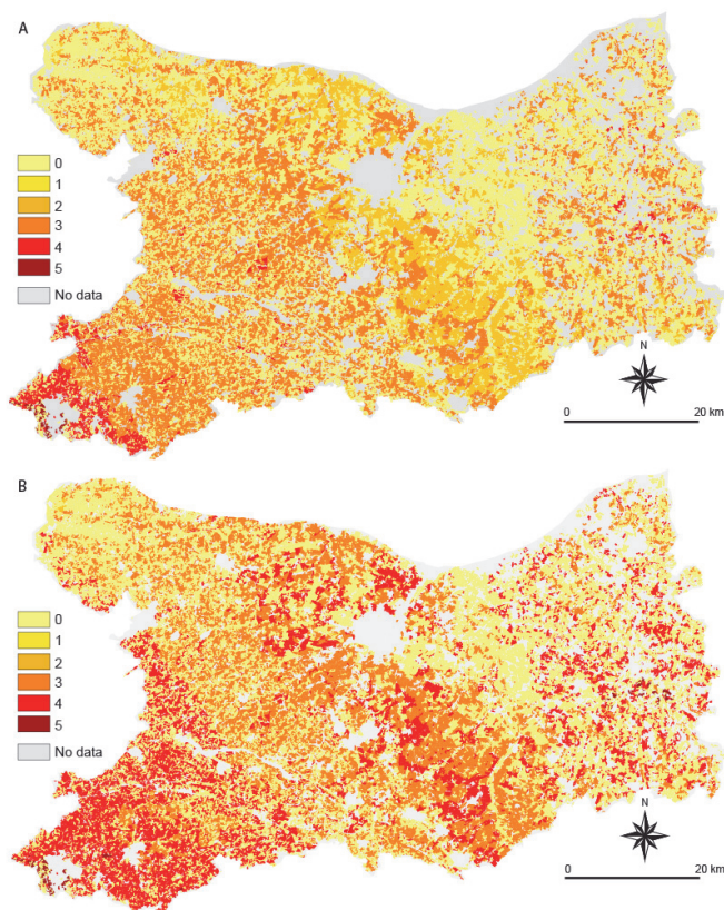
Fig. 6. Soil erosion hazard in Calvados at parcel scale (A) for a normal climatic context, (B) for a rainy year
