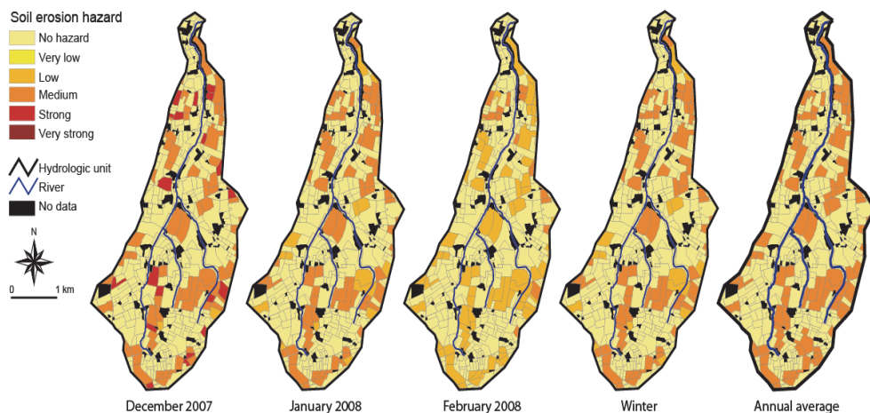
Fig. 11. Maps of soil erosion hazard at various temporal scales.
