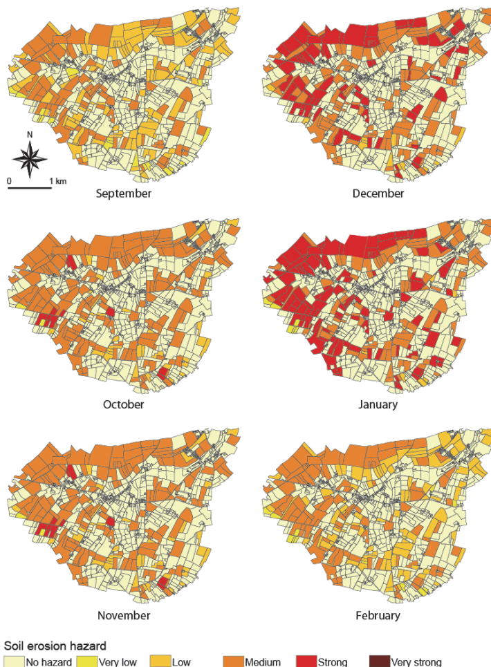
Fig. 13. Maps of soil erosion hazard in current climatic context at monthly scale.
