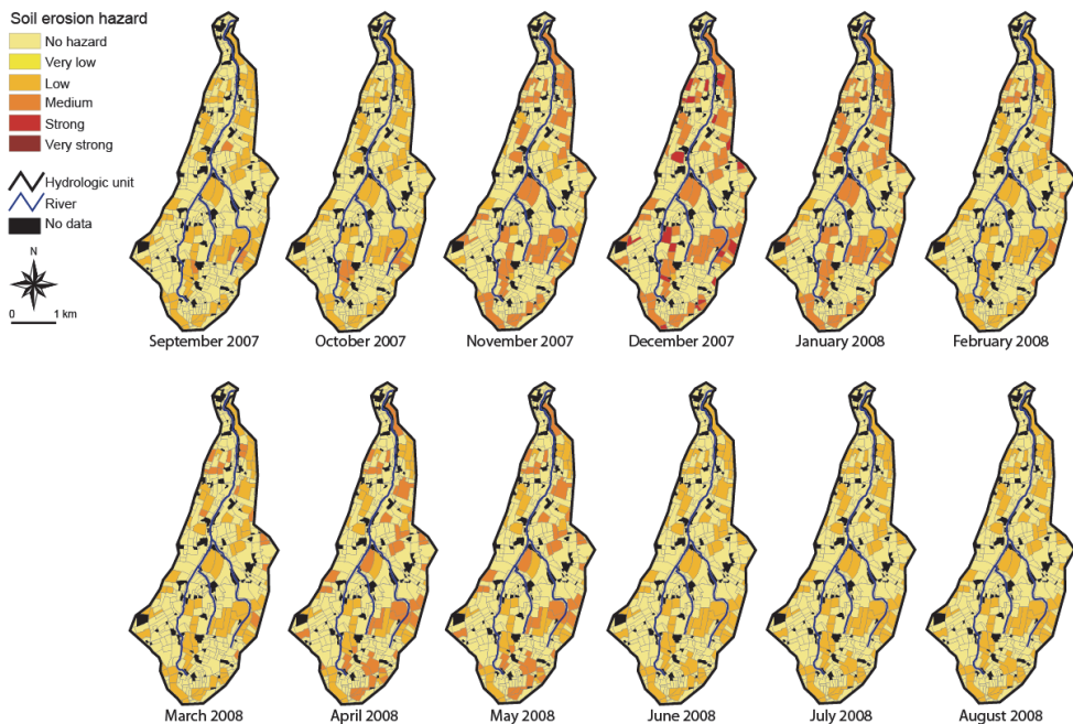
Fig. 9. Maps of soil erosion hazard at monthly scale.
