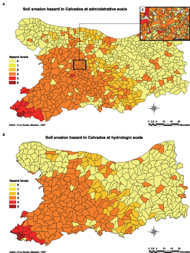
Fig. 7. Aggregation of the soil erosion hazard data: (A) at the administrative scale (municipality); (B) at the hydrologic scale; (C) significant deterioration of results from the parcel scale to the administrative scale due to aggregation procedure
