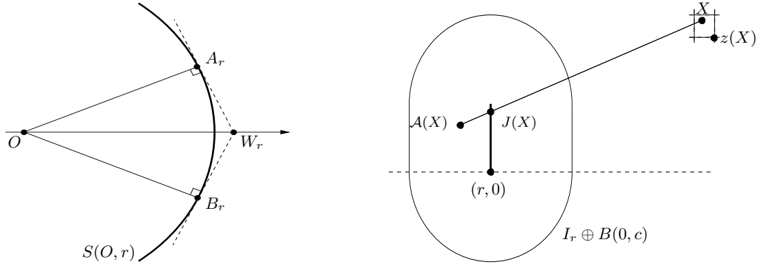
Figure 2: On the left: The sphere S(O, r) with center O and radius r is represented in bold. The tangents (the dotted lines) to S(O, r) respectively at A_r and B_r , intersect the horizontal axis on W_r . On the right: The segment [X, \mathcal{A}(X)] crosses I_r (in bold) on J(X) . On this picture, X is outside I_r \oplus B(0, c) .
