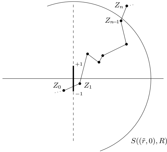
Figure 1: Here is the sub-path Z_0, \dots, Z_n of the RST crossing the vertical segment \{\tilde{r}\} \times [-1, 1] (in bold) and the sphere S((\tilde{r}, 0), R) . On this picture, Z_0 and Z_n belong to B((\tilde{r}, 0), 2R) which occurs with high probability.
