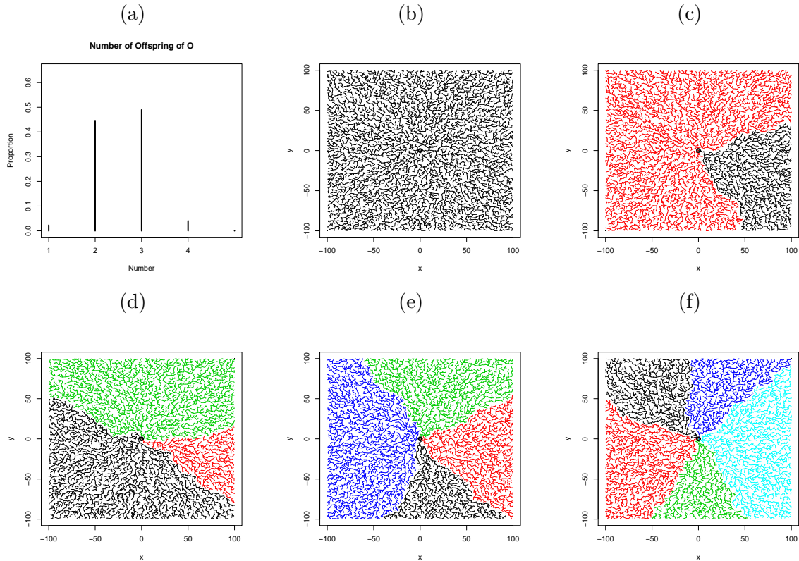
Figure 3: (a) Empirical distribution for the number of children of O . Over 5000 simulations, 1 (resp. 2, 3, 4 and 5) child is obtained in 114 (resp. 2232, 2449, 203, 2) cases. Simulations of m = 1, \dots, 5 subtrees of the RST rooted at the children of O are given from (b) to (f). They seem to be unbounded.
