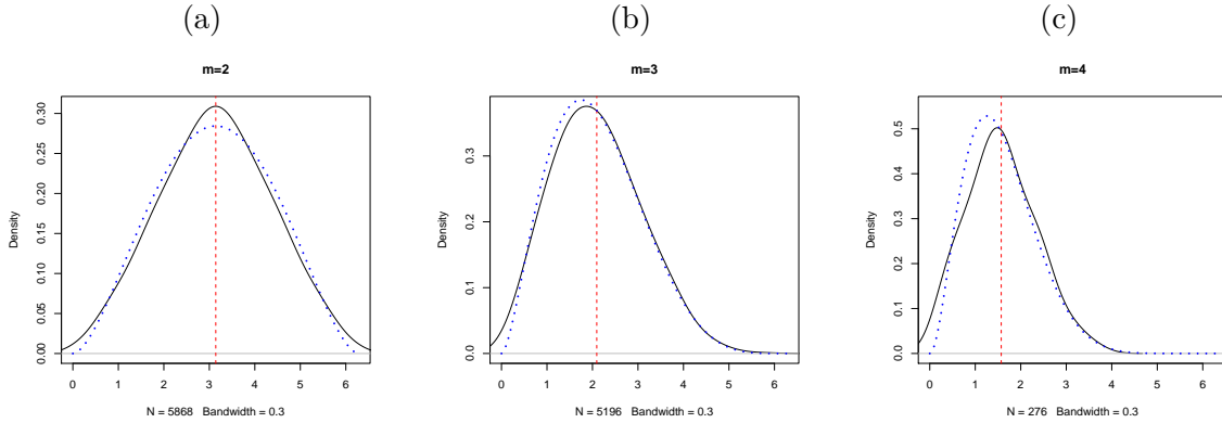
Figure 6: Density estimation for the angles between two interfaces, given the number m of unbounded trees. Given m , the distribution concentrates around 2\pi/m (red dashed line) and has a smaller variance for greater m 's. Calibration with Beta distributions have been carried (blue dotted thick line), but KS test (with test statistic D ) rejects the null hypothesis of Beta distribution B(\hat{\alpha}, (m-1)\hat{\beta}) in the three cases with p -values smaller than 2.2e-16 although the distributions look similar graphically. (a) \hat{\alpha} = \hat{\beta} = 2.74 , D = 96\% ; (b) \hat{\alpha} = 2.69 , \hat{\beta} = 5.38 , D = 91.77\% ; (c) \hat{\alpha} = 2.99 , \hat{\beta} = 8.99 , D = 88.79\% .
