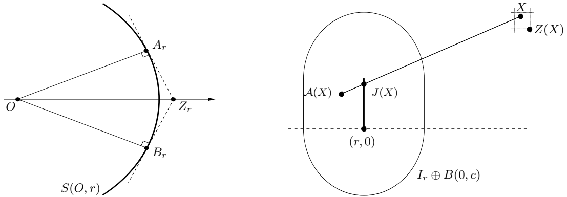
Figure 2: On the left: The sphere S(O, r) with center O and radius r is represented in bold. The tangents D_r and D'_r (the dotted lines) to S(O, r) respectively at A_r and B_r , intersect the horizontal axis on Z_r . On the right: The segment [X, A(X)] crosses I_r (in bold) on J(X) . On this picture, X is outside I_r \oplus B(0, c) .
