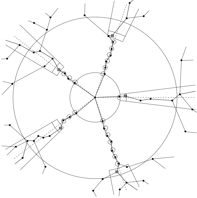
Figure 5: RST of the PPP N satisfying both events A_\varepsilon(r_1, \dots, r_5) and B_\varepsilon(r_1, \dots, r_5) . Beware the fact that, in order not to overload the figure, the condition (\diamond) of B_\varepsilon(r_1, \dots, r_5) has not been represented. The two balls are centered at O with radii r = \min_{k \in \{1, \dots, 5\}} r_k and R = \max_{k \in \{1, \dots, 5\}} r_k + 1 . The X_k 's are represented by big gray squares while the other points of N by small black circles.
