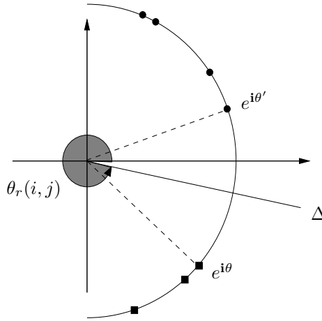
Figure 4: On the unit sphere, the black squares are points of \mathbf{T}_r(i) while black circles are points of \mathbf{T}_r(j) . The arc a(\theta, \theta') is divided in two equal parts by the line \Delta whose angle (represented in grey) is \theta_r(i, j) .
