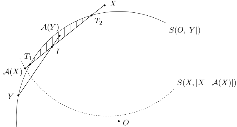
Figure 7: The hatched area corresponds to the one of the two sets U and V which is included in the ball B(X, |X - \mathcal{A}(X)|) . Here, it contains \mathcal{A}(Y) . Besides, let us remark the origin O cannot belong to the ball B(X, |X - \mathcal{A}(X)|) .
