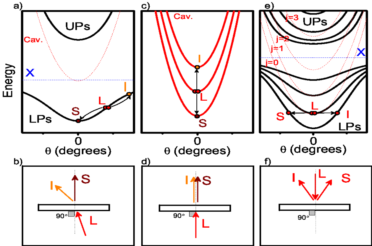
Figure 1 a) Thin lines are exciton (X) and cavity photon (Cav) dispersions. Thick lines are UP and LP dispersions. Arrows indicate the intraband parametric process. b) Scheme of the PSP: the excitation laser is tilted with respect to the normal to the sample surface while signal S and idler I are split. c) Photonic band dispersion of a triply-resonant 2D-MC and corresponding interbranch PSP split in energy and degenerate in momentum space. d) Corresponding scheme of the PSP with laser normal to the sample surface and degenerate S and I. e) Thin lines are photonic band dispersion and exciton states. Thick lines are multi-branch UP and LP states. Arrows show an interbranch PSP degenerate in energy and split in momentum. f) Scheme of the PSP with laser normal to the sample surface and mirror-symmetric S and I.
