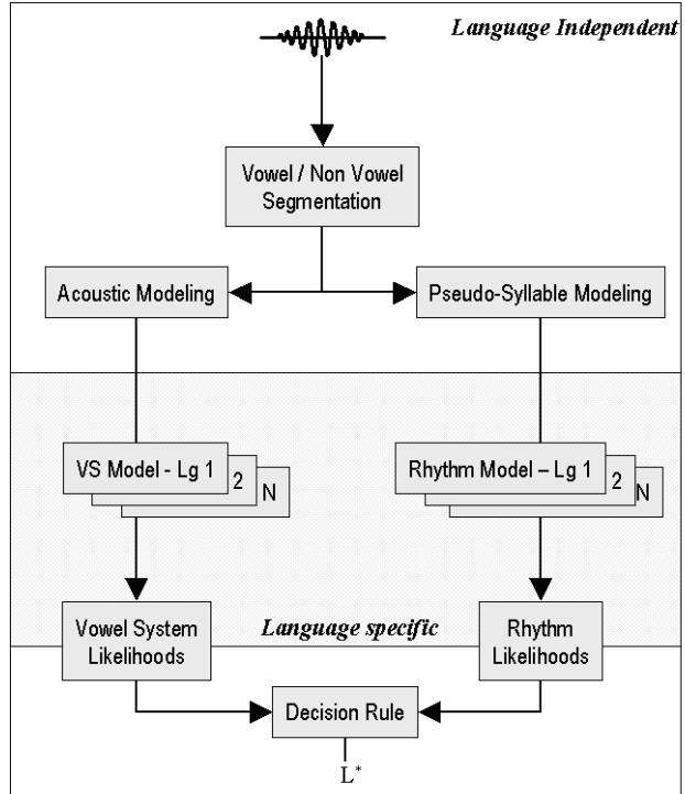
Figure 1 - Synopsis of the system for N languages.
