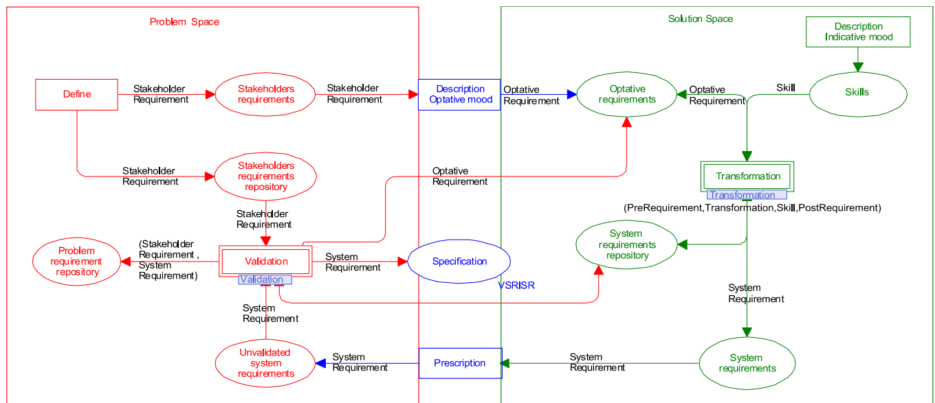
Fig.5. Main structure of the iterative workflow proposed for RS
