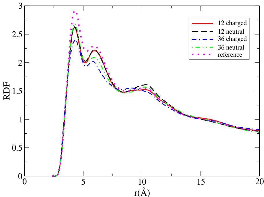
Figure 8: The radial distribution function between carbonyl oxygens of the two lipid tail chains (OH and OF)
