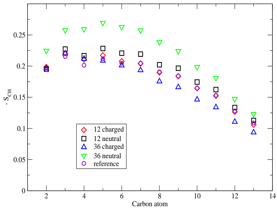
Figure 5: CH bond order parameters for different carbon atoms in the sn 1 chain of lipids
