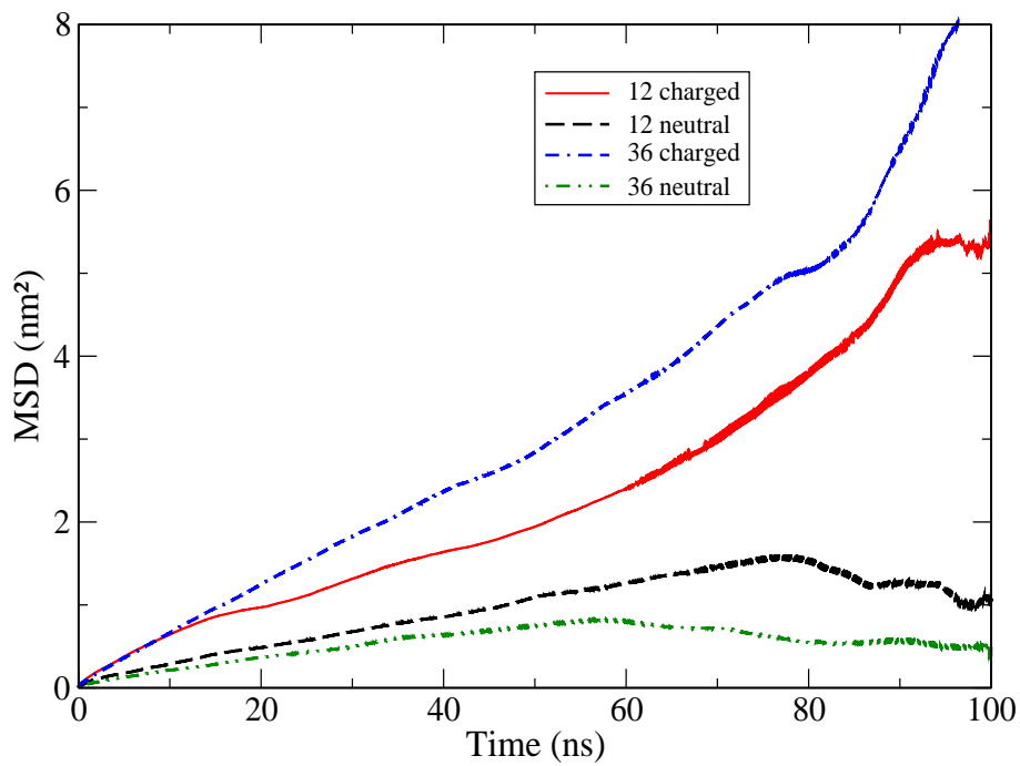
Figure 9: Lateral mean square displacement of articaine.
