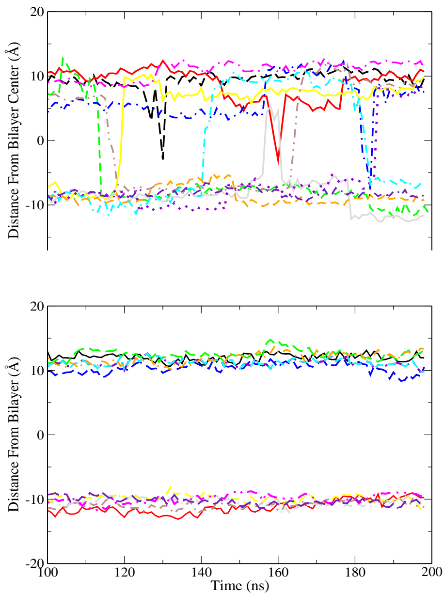
Figure 10: Distance from the bilayer center to the centers of mass of 12 uncharged (a) and 12 charged (b) artocaine molecules as a function of time. Different molecules are represented by different colors and line styles.
