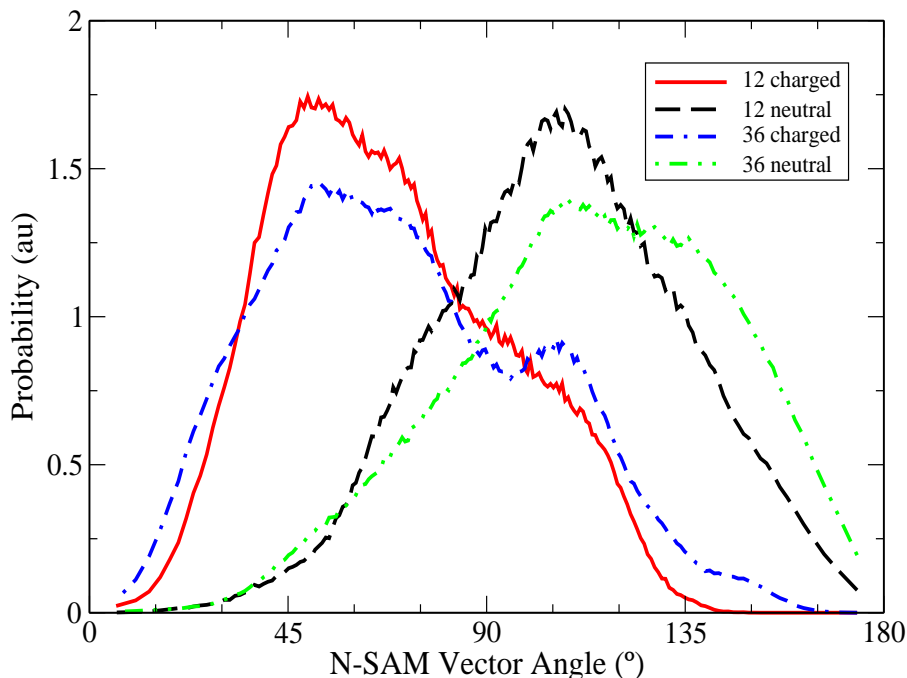
Figure 4: Angular distribution of the N-SAM vector of articaine molecules in the DMPC bilayer relative to the bilayer normal
