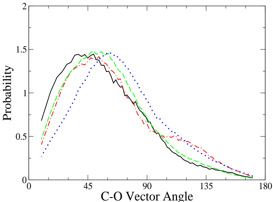
Figure 12: Probability distribution of the angle between outward direction of the bilayer normal and carbonyl bond C-O (black solid and green dashed lines) and CAN-OAE (red dash-dot and blue dot lines) of neutral artocaine molecule. System with 12 artocaine molecules: black solid and red dash-dot lines; system with 36 artocaine molecules: green dashed and blue dot lines.
