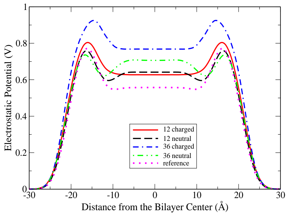
Figure 11: Membrane electrostatic potential
