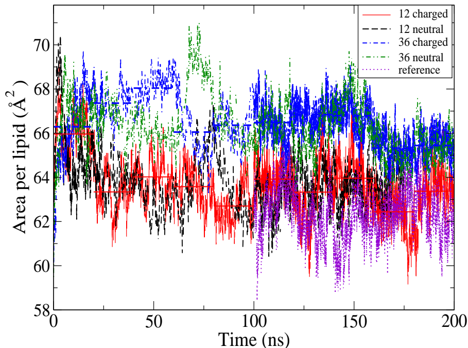
Figure 2: The time evolution of the area per lipid for the simulated systems. For charged systems, averages over 20 ns time intervals are shown as horizontal lines.
