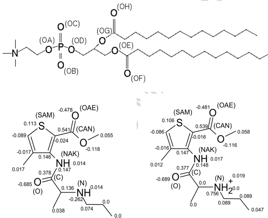
Figure 1: Molecular structure of DMPC lipid (top), neutral (bottom left) and charged (bottom right) forms of articaine, with partial atom charges and atom names referred in the text
