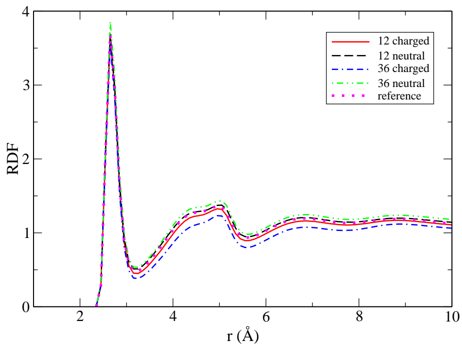
Figure 7: The radial distribution function of water oxygen around phosphate oxygen (OB and OC) of DMPC lipid molecules
