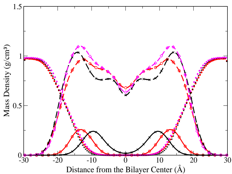
Figure 3: Mass density of different components as a function of distance from the bilayer center for 36 articaine molecules and for the reference bilayer. Charged articaine system: red lines with circles; uncharged articaine system: black lines with crosses; reference system: magenta lines with diamonds. Mass density of articaine: solid lines; DMPC: dashed lines; water: dotted lines.
