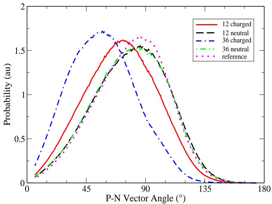
Figure 6: Distribution of the angle between P-N vector of DMPC head group and the outward normal of the bilayer
