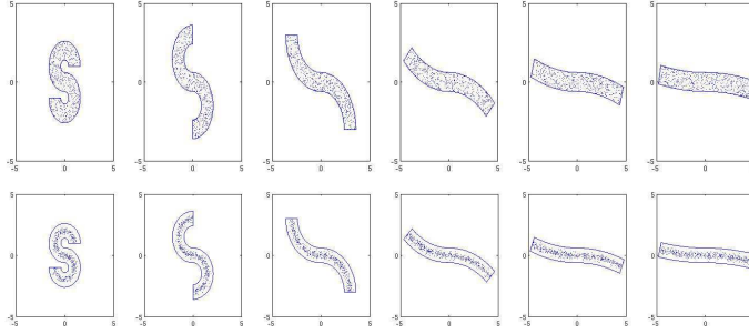
FIG 2. S_R for different values of R . sample is also presented, drawn with a uniform radial noise (top) and with a truncated Gaussian noise (bottom)
