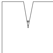
FIG 1. [0, 1]^2 \setminus T_\varphi where T_\varphi is an isosceles triangle with height 1/2.
