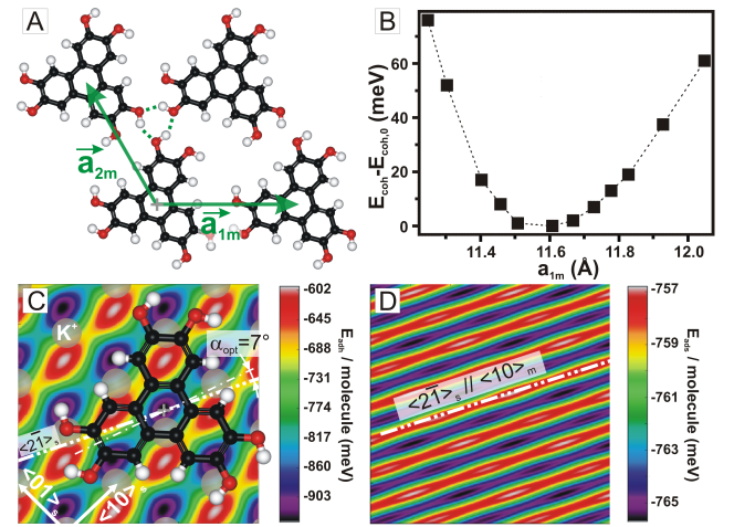
FIG. 3: (Color online) A- Unit cell of the HHTP freestanding layer as calculated by DFT. A H-bonded (dotted green lines) hexagonal structure with \|\mathbf{a}_{1m,2m}^{\text{DFT}}\| = 11.62 Å is found. B- Evolution of the cohesion energy per molecule as a function of a_{1m}^{\text{DFT}} (uniaxial stress), from which the uniaxial stiffness k_{\text{DFT}} = 15.3 N/m of the layer is derived. C- Adhesion energy of a single HHTP adsorbed on KCl(001), as calculated by PE calculations. The constant background of -0.76 eV (mainly vdW interaction) is laterally corrugated due to ES molecule/substrate interaction. D- Adsorption energy per molecule for a cluster of 3600 molecules when translated with fixed angular orientation. The remaining 1D potential is 4 meV deep and carries the lol epitaxy direction.
