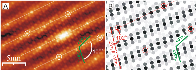
FIG. 2: (Color online) A- Autocorrelation image of a molecular domain showing Moiré fringes and periodic bright spots. The orientation of the fringes w.r.t. \langle 10 \rangle_m is (100 \pm 3)^\circ . B- Simulated Moiré pattern which reproduces both the experimental fringes and the bright spots, respectively.
