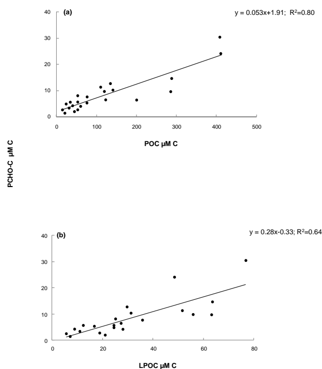
Fig. 2. Relationships between PCHO-C and (a) POC; (b) LPOC during the sampling period (May 2007–June 2009). Labile POC was calculated as follows: 0–15 mg l -1 TSM corresponds to 35.2 % LPOC; 15–50 mg l -1 TSM, 46.60 % LPOC; 50–150 mg l -1 TSM, LPOC 22.10 %; 150–500 mg l -1 TSM, 11.8 % LPOC; 500–1500 mg l -1 TSM, 18.8 % LPOC (Ittekkot, 1988).
