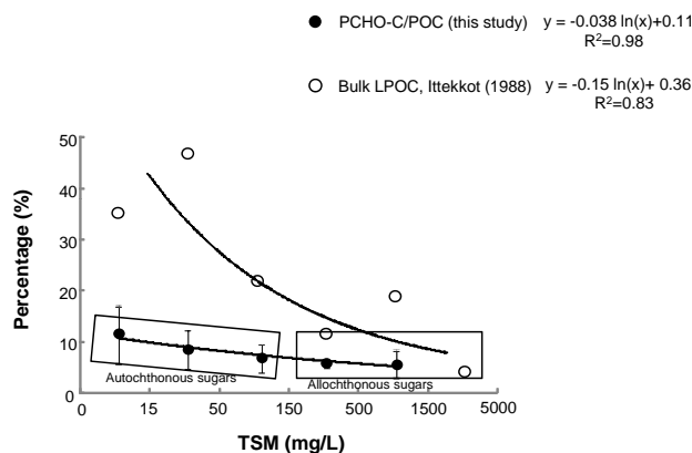
Fig. 3. The percentage of labile POC as a function of the TSM concentrations. In our study, the Rhône River TSM concentrations ranged between 6 and 1044 mg l -1 ; therefore, TSM > 1500 mg l -1 are not available. The error bars represent the standard deviation of the TSM concentrations for the range of 0–15, 15–50, 50–150, 150–500, and 500–1500 mg l -1 , as established by Meybeck (1982).
