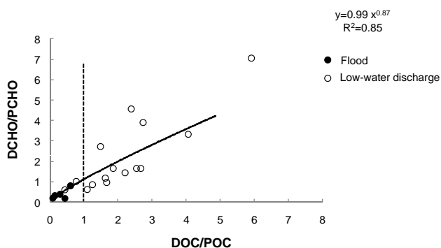
Fig. 5. Relationship between the ratios DCHO/PCHO and DOC/POC during the sampling period. We considered a flood event to occur when Q > 3000 \text{ m}^3 \text{ s}^{-1} . This value roughly corresponded with two times the average annual flow recorded in the Rhône River ( Q \approx 1500 \text{ m}^3 \text{ s}^{-1} ).
