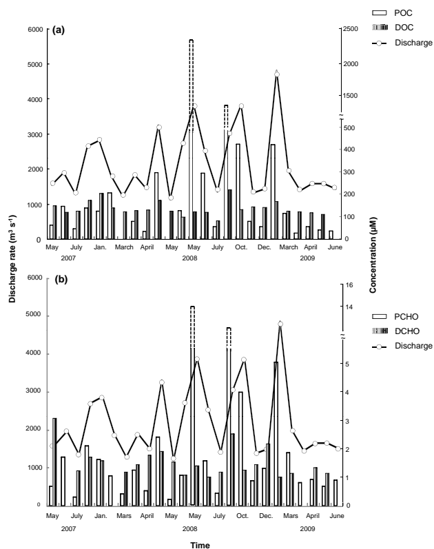
Fig. 1. Daily discharge of the Rhône River (in \text{m}^3 \text{s}^{-1} ) between May 2007 and June 2009 as a function of (a) POC and DOC concentrations (in \mu\text{M} C) and (b) PCHO and DCHO concentrations (in \mu\text{M} ).
