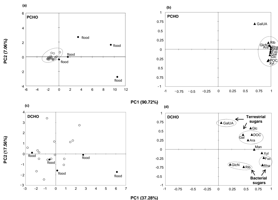
Fig. 4. Principal components analysis for particulate and dissolved carbohydrates, including POC and DOC. (a) and (c) are the sample scores, whereas (b) and (d) are the sample loadings of the PCA. The variance accounted for by each principal component is shown in parentheses after the axis label. The abbreviations of the sugars are given in Table 2.
