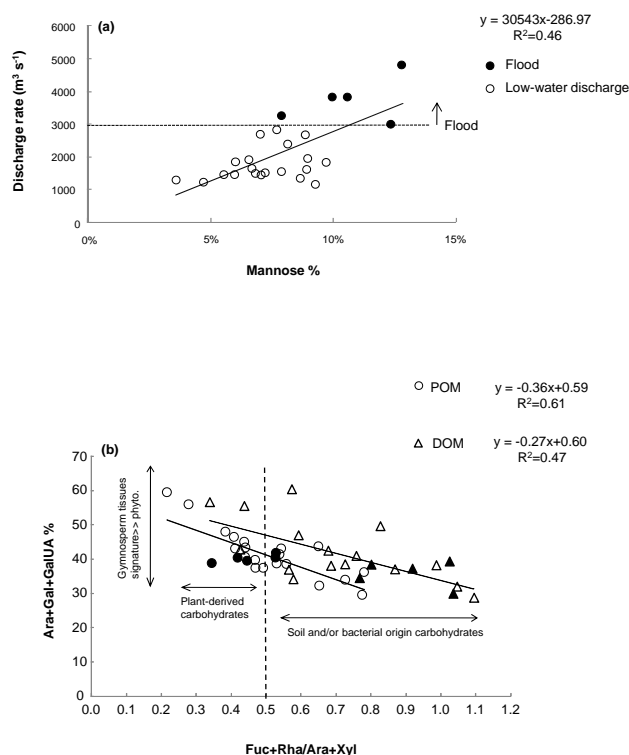
Fig. 6. (a) Relationships between mannose and discharge in POM and (b) relationships between the ratio \text{Fuc} + \text{Rha}/\text{Ara} + \text{Xyl} and \text{Ara} + \text{Gal} + \text{GalUA} (%) in POM and DOM over the sampling period. Flood events are indicated as bold circles and triangles.
