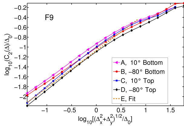
Figure 12: Plot of \log_{10} [C_2(\Delta)/\Delta_0] as a function of \log_{10} [\Delta/\Delta_0] , computed for discontinuity F9, in directions \theta equal to 10^\circ and 80^\circ , for the bottom side (A, B) and top side (C, D), respectively. Plot E is a linear fit \log_{10} [C_2(\Delta)/\Delta_0] = 0.75 \log_{10} [\Delta/\Delta_0] - 1.07 , i.e. \zeta = 0.75 and C_2(\Delta_0) = 0.09 mm, plotted from \Delta = 40 \mu\text{m} to \Delta = 7 mm. \Delta and C_2 are in mm, and \Delta_0 = 1 mm.
